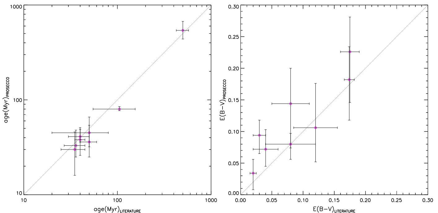
Fig. 12. Ages (left-hand panel) and reddening (right-hand panel) derived in this work using PROSECCO models vs. values from the literature (see Table 1).
