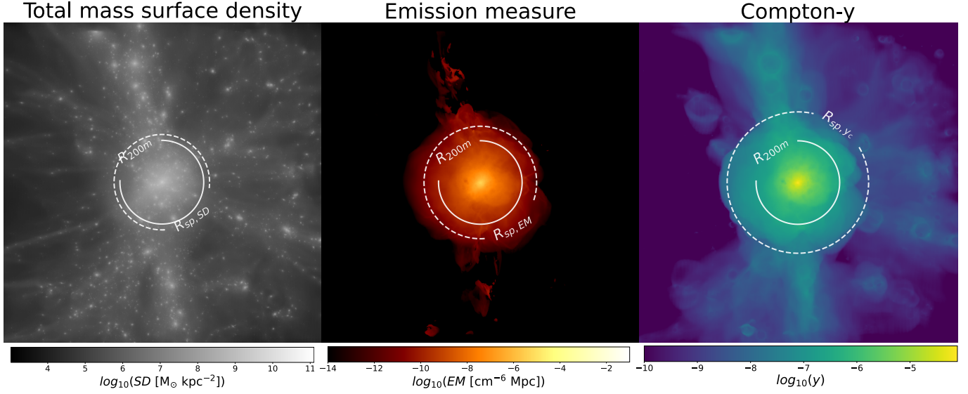
Fig. 1. Projected maps of SD (left), EM (centre), and Compton- y (y, right). The projection follows the direction between the Milky Way’s assumed position and the Virgo cluster’s centre. The maps are 22.122 Mpc wide and contain 15\,728^2 pixels. The circles represent R_{200m} (solid white) and R_{sp} (dashed white) identified in each 2D-projected profile extracted from the maps.
