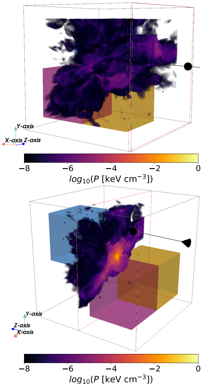
Fig. 2. 3D visualisation of the pressure in the Virgo replica simulation. The pressure is in \text{keV} \cdot \text{cm}^{-3} and is shown on a log scale in the range of [-8, 0] . The top panel shows the full box and the bottom panel shows a slice in the cluster's core along the z axis. The orange sub-box is the region of outflowing material, the blue sub-box is the region of collapsing material, and the pink sub-box is the region of filament material.
