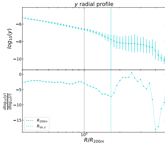
Fig. 9. Projected radial profiles of Compton-y. The profile is shown in the top sub-panel, and its gradient is shown in the bottom sub-panel. The dashed vertical lines represent R_{200m} (grey) and R_{sp} (turquoise) identified in the 2D-projected profiles extracted from the Compton-y maps.
