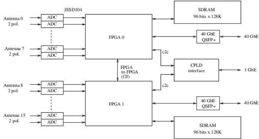
Fig. 3. Tile Processing Module Structure
