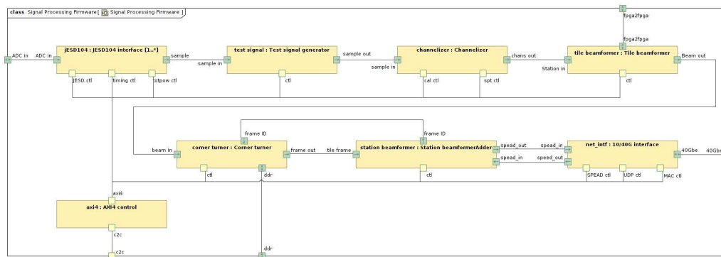
Fig. 6. Firmware - Block Definition Diagram
