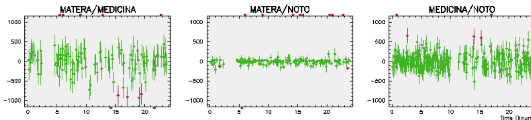
Fig. 1 SOLVE residuals from the first Italian geodetic VLBI experiment.
