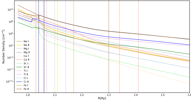
Fig. 8. Number densities predicted by the NLTE model of Fossati et al. (2021) for the detected atoms in neutral and singly ionised form. The dashed lines indicate the height probed by the observations. Generally, the ionised species have higher number densities compared to the neutral ones.
