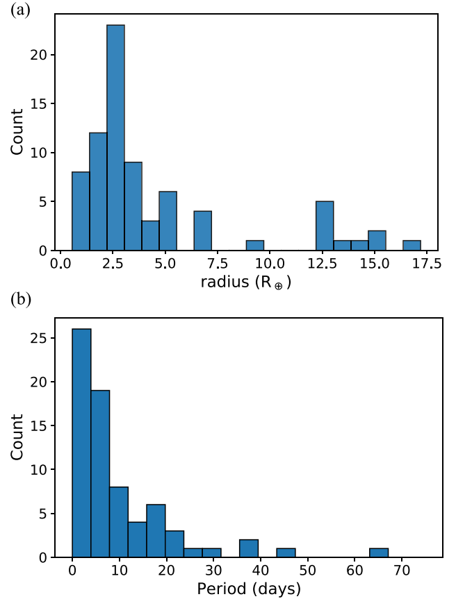
Figure 4. Most of the planets in our sample are small ( 1\text{--}5 R_{\oplus} ), and thus have relatively low false-positive probabilities (e.g., Morton & Johnson 2011; Guerrero et al. 2021) compared to giant planet candidates (Santerne et al. 2012).
