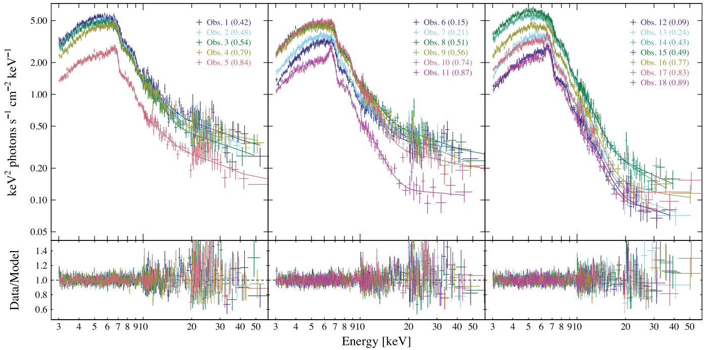
Fig. 8. NuSTAR spectra with \sim 1 msec exposure through the whole pointing spanning \sim 2.5 orbits. Orbital phase is indicated in parenthesis ( left panel : first half orbit, middle panel : second orbit, right panel : third orbit). The spectra are fitted with a model consisting of absorbed blackbody, Comptonization, and Gaussian components multiplied by three absorption edges from neutral and ionized iron. The model residuals are shown in the bottom panels. The plotted spectra are from FMPA for clarity, but the models are fitted to both detectors simultaneously.
