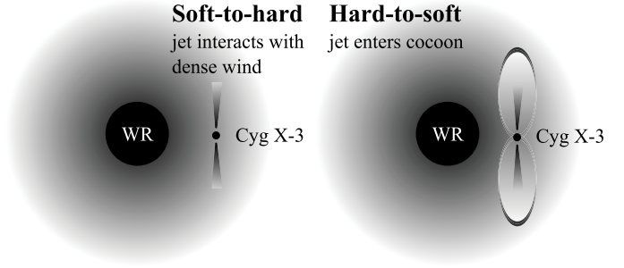
Fig. 13. Cartoon of the jet-wind interaction for Cyg X-3. Left: in the hypersoft state the jet is turned off and the stellar wind is allowed to expand freely close to the compact object. When the jet turns back on during the state transition, it encounters a dense medium at rest relative to the jet which leads to efficient shock production and subsequently to strong radio and \gamma -ray emission. Right: when Cyg X-3 is transiting from the hard state to the hypersoft state, the hard state compact jet has blown out a cocoon in the stellar wind, into which the episodic jet can then expand more freely producing weaker radio emission than when expanding directly into a stellar wind. We note that the stellar sizes and the binary separation are not to scale with respect to the jet.
