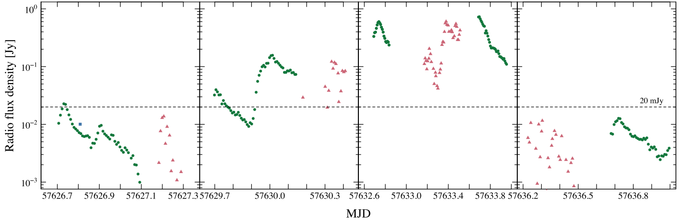
Fig. 2. Intraday radio light curves (green: 15 GHz, red: 230 GHz) from the 2016 hypersoft state ( first and last panels ) and minor radio flare ( middle panels ). The colors are same as in Fig. 1. The 230 GHz light curve seems to present higher variability (see Fig. 3 and 4). The 15 GHz light curve presents some well-defined flares that last \sim 0.1 days, indicating a size scale of 3 \times 10^{14} cm (well beyond the orbital scale).
