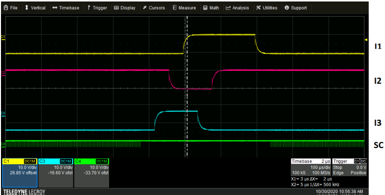
Figure 16 - Vertical waveforms with 0.1 µF capacitor filter in the intermediate board
