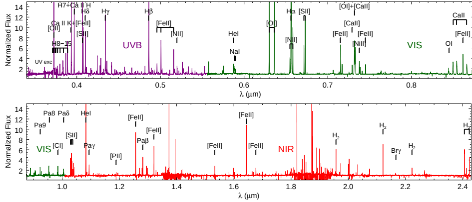
Fig. 1. X-Shooter spectrum of the pre-main sequence object Sz102 (Antonucci et al., in prep.). The main emission features detected, which trace different structures of the source (see text), are indicated.
