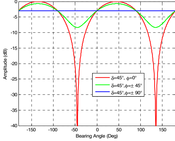
Fig. 5. Amplitude response for a complete spin-flight at zenith ( \theta=0^\circ ) for three values of the parameter \varphi .
