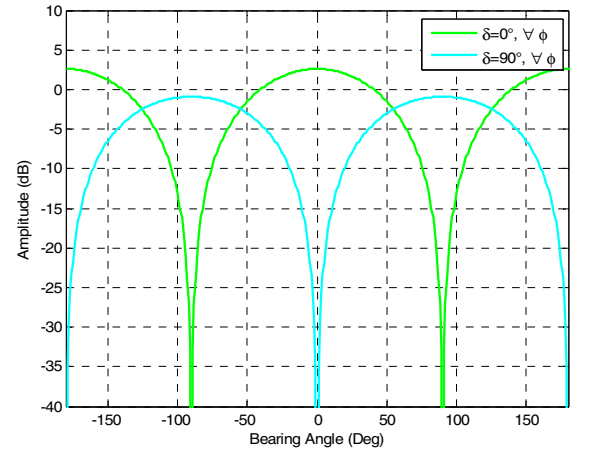
Fig. 6. Amplitude response for a complete spin-flight at zenith ( \theta=45^\circ ) for two values of the parameter \delta .
