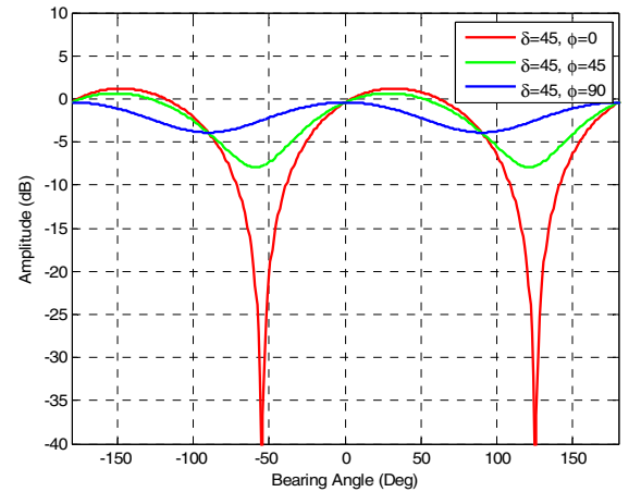
Fig. 7. Amplitude response for a complete spin-flight at zenith ( \theta=45^\circ ) for two values of the parameter \varphi .
