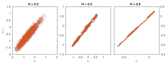
FIG. 7. Phase-space portraits of three realizations of fractional Brownian motion with Hurst exponents H = 0.2, 0.5 , and 0.8 (left to right) as obtained from the raw time series [(x_t, x_{t+1})] , gray and from reconstructions of empirical modes [(x_t^*, x_{t+1}^*)] , orange.
