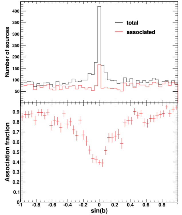
Figure 19. Upper panel: Distributions in Galactic latitude b of 4FGL sources (black histogram) and associated sources (red histogram). Lower panel: Association fraction as a function of Galactic latitude.
