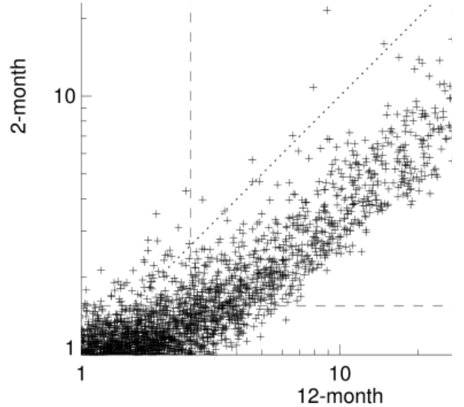
Figure 12. Comparison of the reduced variability index (divided by N_{\text{int}} - 1 ) from two-month intervals with that for one-year intervals. This illustrates that, for the majority of sources (AGN characterized by red noise) using longer intervals detects variability better. The dotted line is the diagonal (expected for white noise). The dashed lines show the two variability thresholds.
