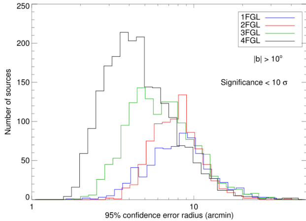
Figure 18. Distributions of the 95% confidence error radii for high-latitude sources with significance < 10\sigma in 1FGL (713 sources, blue), 2FGL (843 sources, red), 3FGL (1387 sources, green) and 4FGL (2090 sources, black), illustrating the improvement of localizations for sources of equivalent detection significances.
