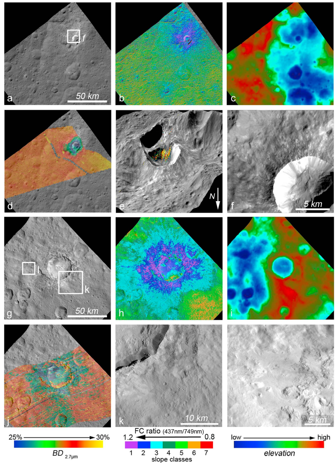
Figure 2. Type localities of blue material: (a) FC image of Oxo, and the corresponding (b) slope classification map (like in Figure 1), (c) DTM, (d) VIR derived BD\ 2.7\ \mu\text{m} map, (e) 3-D view illustrating where \text{H}_2\text{O} ice has been detected, (f) close up FC image of blue ejecta material, (g) FC image of impact crater Haulani, and the corresponding (h) slope classification map, (i) DTM, (j) VIR-derived BD\ 2.7\ \mu\text{m} map, and (k and l) close up FC images of blue-sloped ejecta material.
