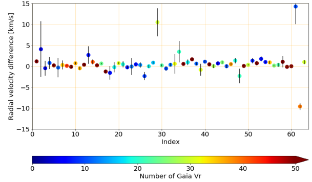
Fig. 25. Difference of mean radial velocities between Gaia and the literature (Dias et al. 2002) for 63 open clusters. The error bars correspond to the quadratic sum of Gaia and literature uncertainties. The abscissa is an arbitrary number of the clusters from 1 to 63. The colour code highlights the number of Gaia members per cluster, which varies from 5 to 191.
