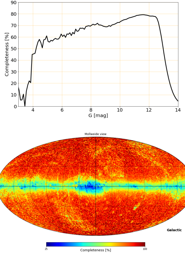
Fig. 6. Top panel: completeness with respect to the full Gaia DR2 catalogue as a function of G magnitude. Bottom panel: completeness with respect to the Gaia DR2 catalogue for the stars with G \leq 12.5 mag as a function of galactic coordinates. The Galactic centre is in the middle of the figure and the Galactic longitudes increase to the left. The pixel size is \sim 0.8 square degree (healpix level 6).
