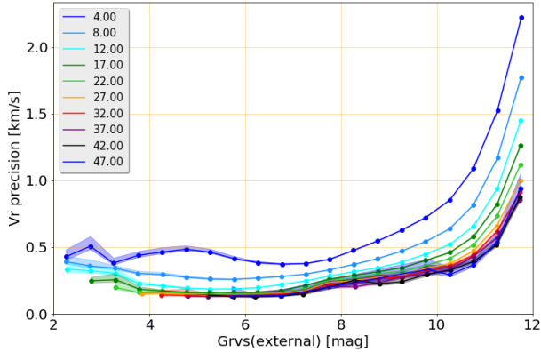
Fig. 18. Radial velocity precision as a function of G_{\text{RVS}}^{\text{ext}} magnitude and number of transits. Each curve corresponds to an interval of five transits: for instance, [2, 6] transits (dark blue), [7, 11] transits (blue). The mean number of transits of each interval is given in the legend. The lower and upper 1\sigma uncertainties on the measures of the precision are represented as shaded areas.
