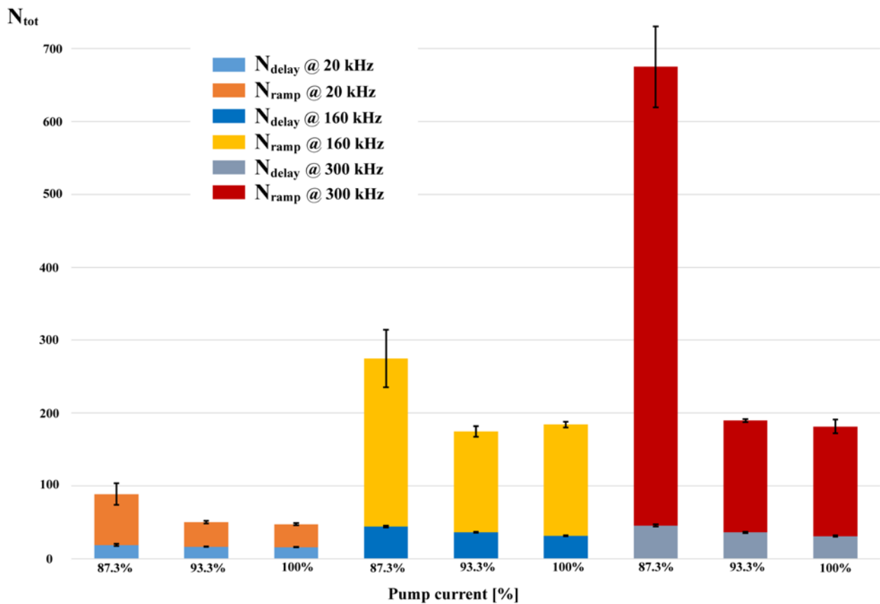
Figure 3 Ramped emission characteristics as function of laser source parameters.
