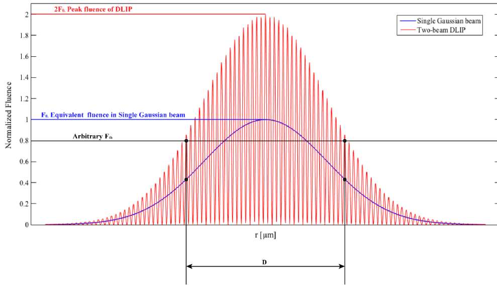
Figure 8 Fluence behaviour considering single Gaussian beam and two-beam DLIP configurations
