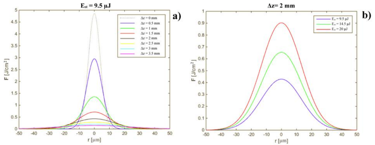
Figure 5 Gaussian profiles: a) constant E_{st} value as a function of different \Delta z , b) constant \Delta z value as a function of different E_{st} levels
