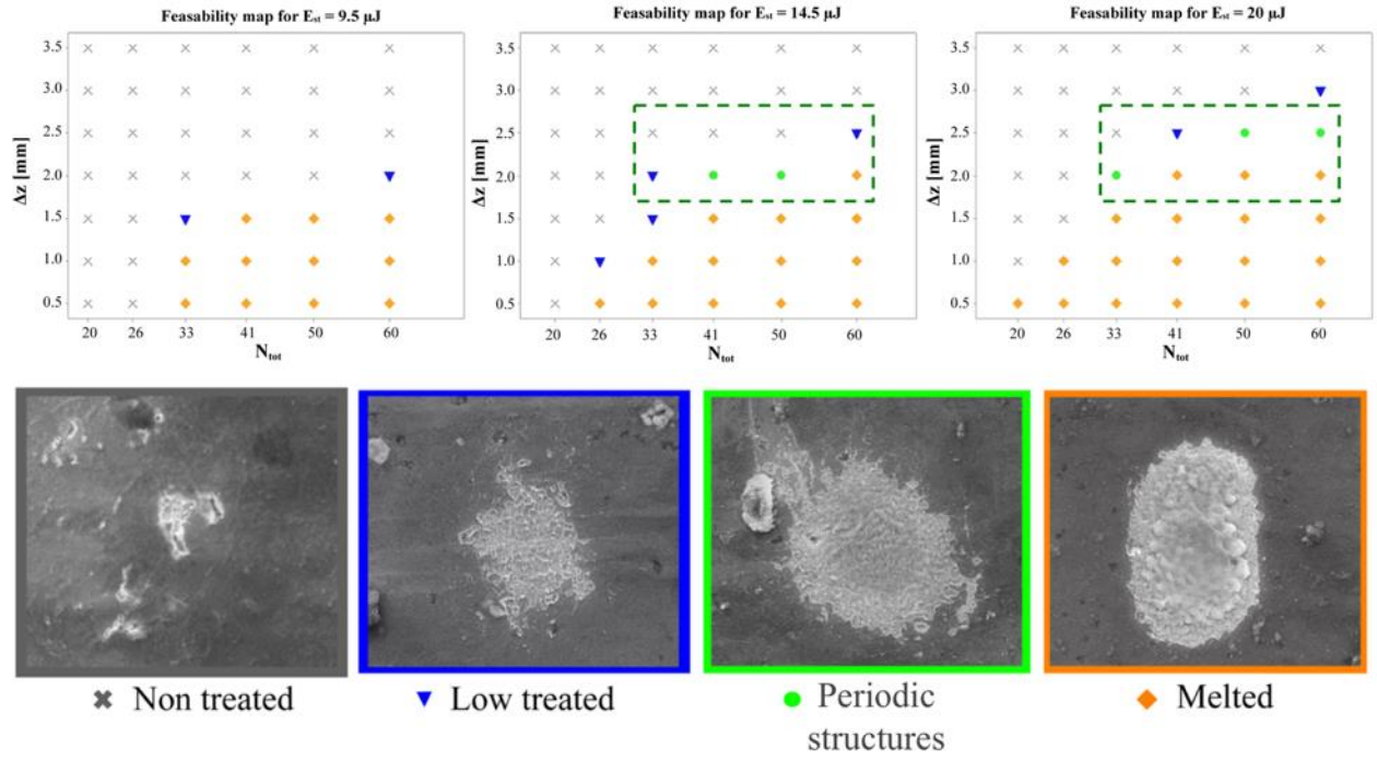
Figure 4 Feasibility map of two-beam DLIP process
