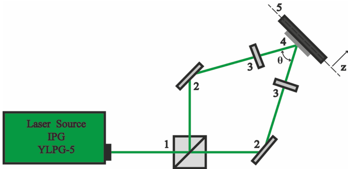
Figure 1 Schematic representation of two-beam DLIP optical setup: 1) beam splitter, 2) mirrors, 3) focal lenses, 4) target plane, 5) z stage
