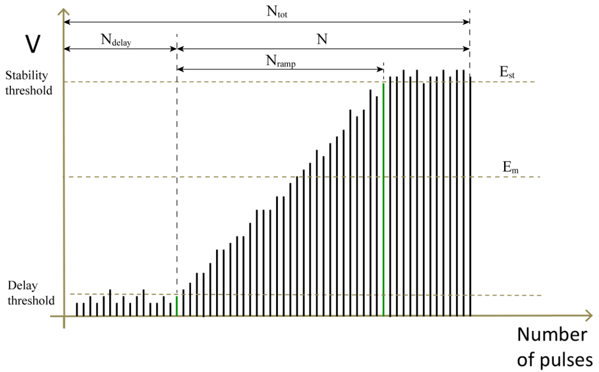
Figure 2 Laser pulsed emission trend for PRR=20 kHz and PI%=100%
