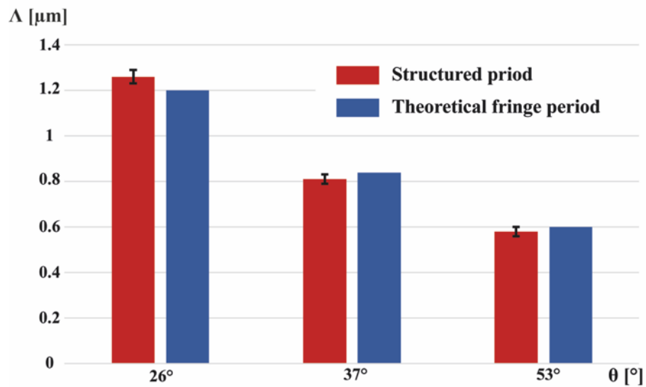
Figure 11 Comparison between measured interference pattern and modelled fringe period
