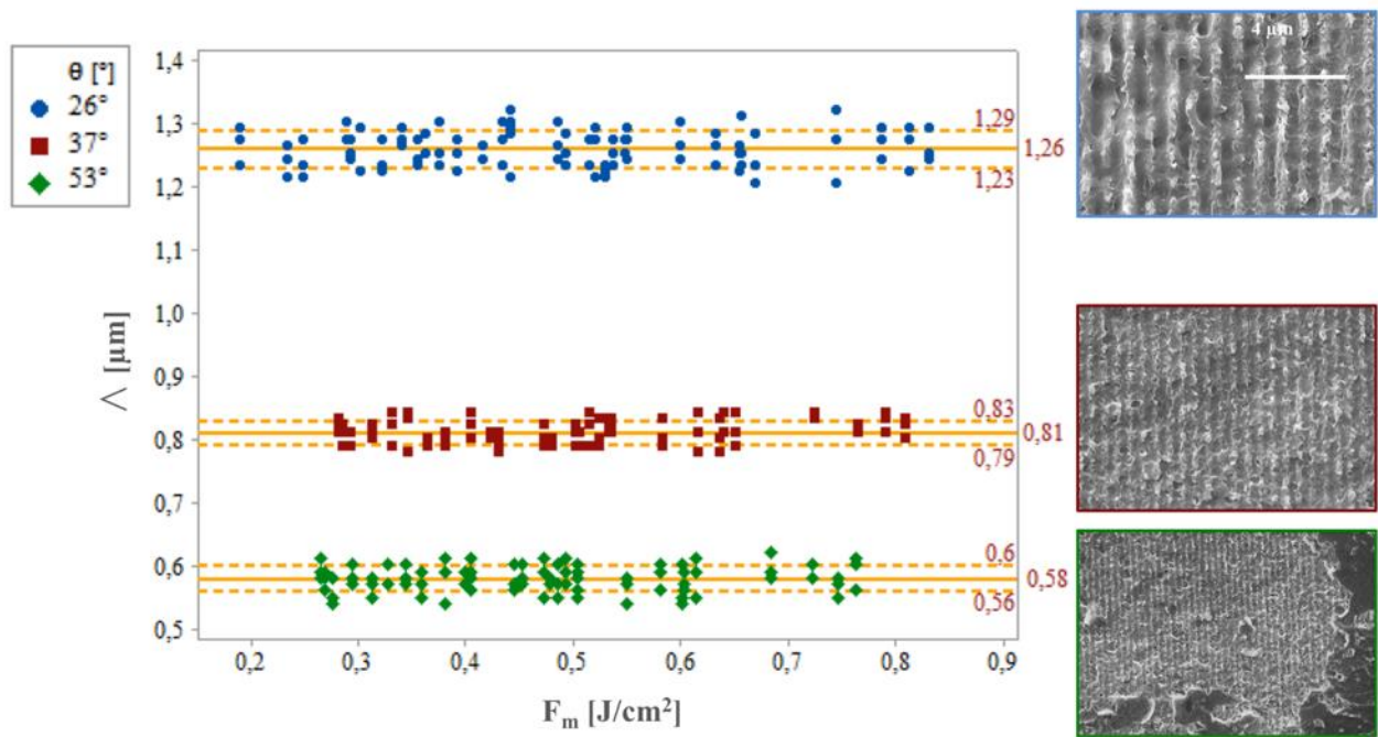
Figure 10 Measured period as a function of average fluence
