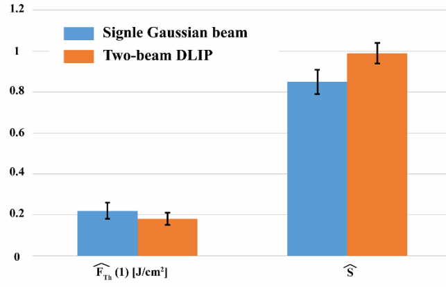
Figure 7. Ablation threshold and incubation coefficient comparison.
