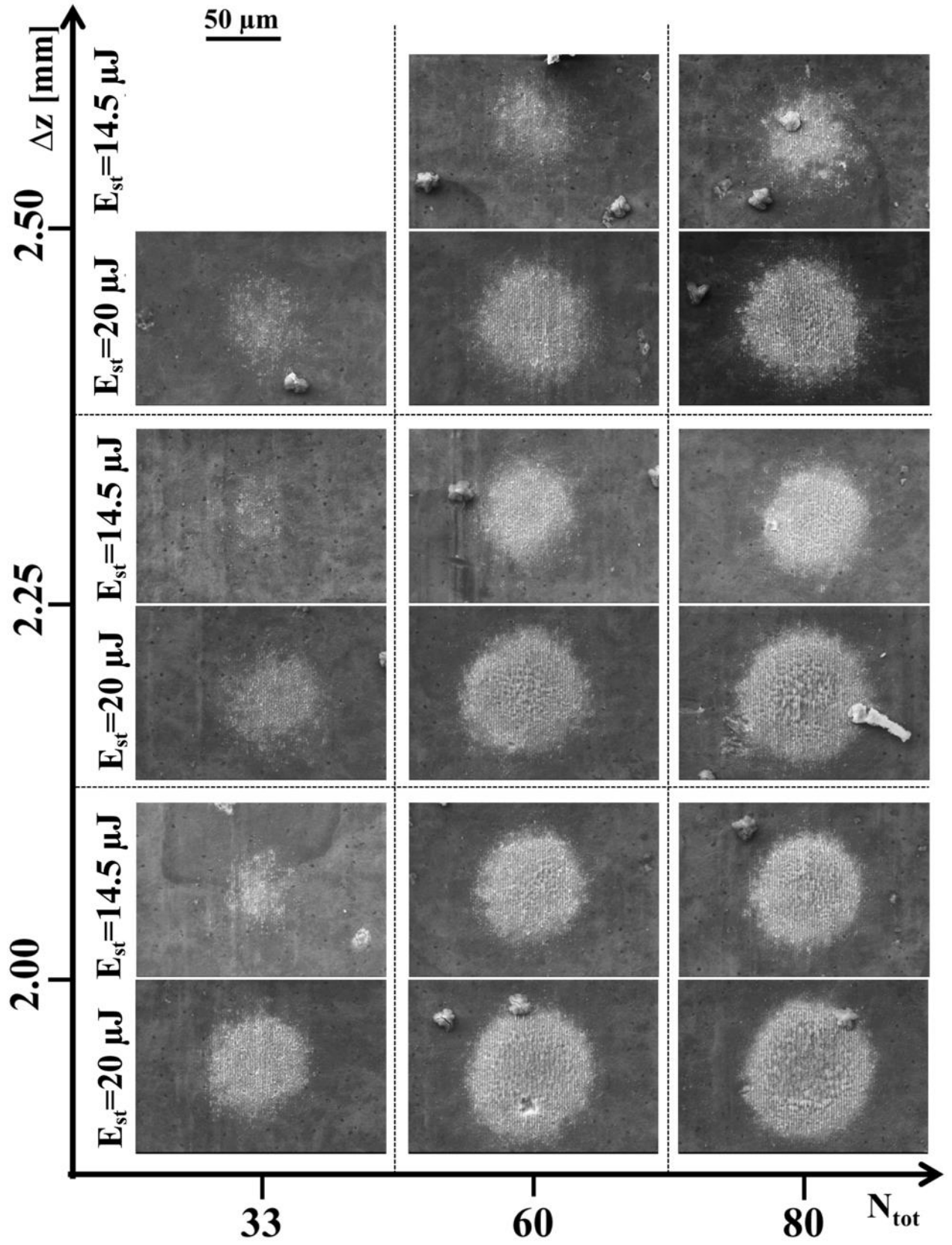
Figure 6 Influence of laser parameters ablated region diameter as function of two-beam DLIP parameters ( \theta=26^\circ ).
