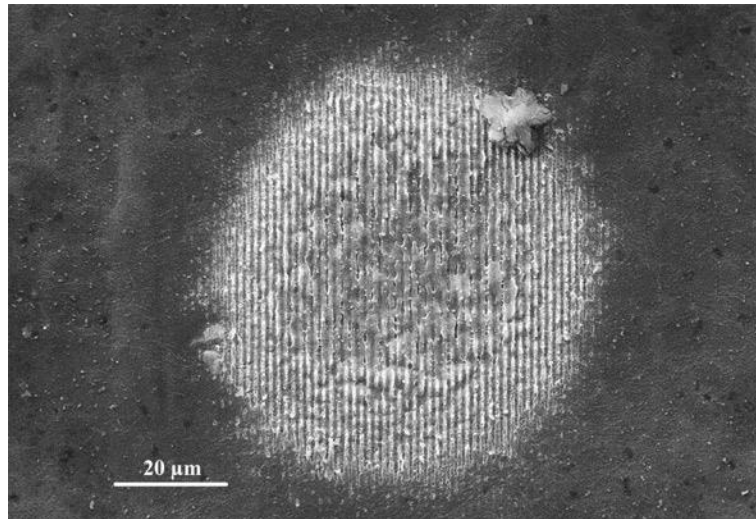
Figure 9 Laser treated spot characterized by E_{st}=20.0 μJ, \Delta z=2 mm, N_{tot}=80 and \theta=26^\circ
