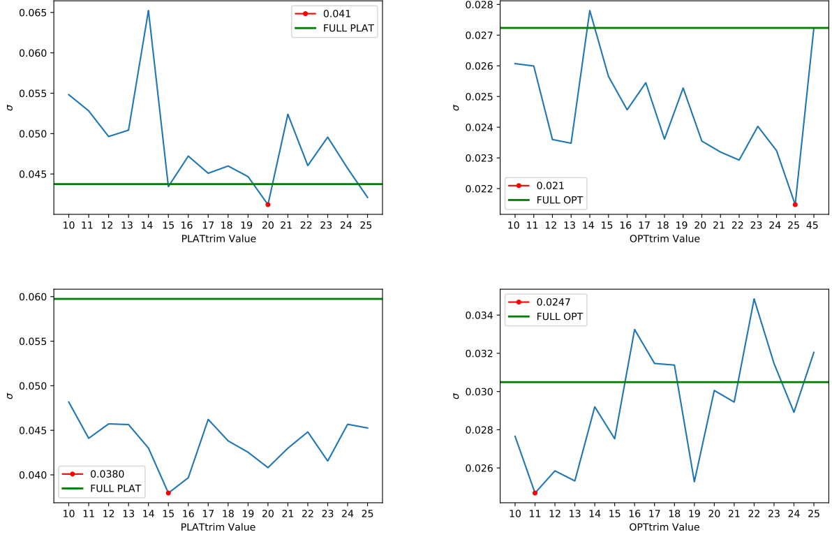
Figure B1. The leftmost plots in this Figure detail the trial simulations for varying PLATtrim values in the X-ray sample, whereas the rightmost plots do the same for varying OPTtrim in the Optical sample. The two upper panels do not consider redshift evolutionary effects; the bottom panels make corrections for both selection and redshift evolution biases.
