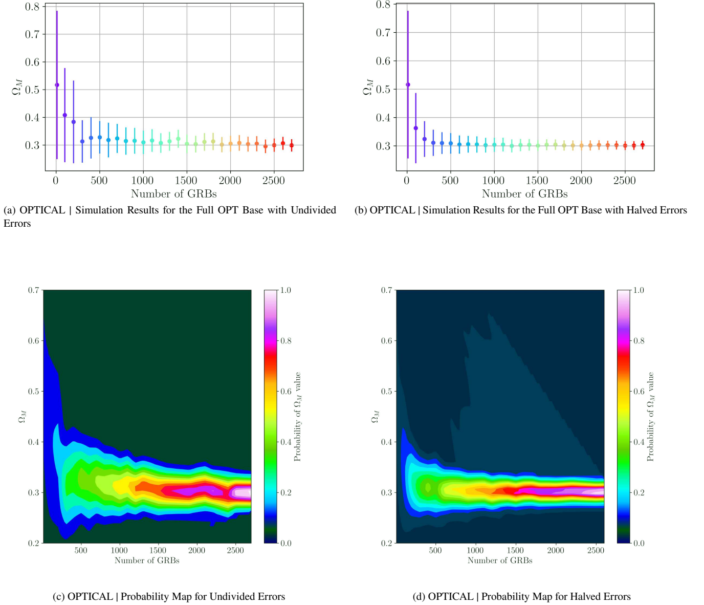
Figure 9. Upper left panel: the mean values of \Omega_M vs. the numbers of GRBs obeying the optical fundamental plane to converge upon a value of \Omega_M using GRBs as the standalone probe by considering the observed error bars. The upper right panel: the same as the left panel, but considering the error bars divided by 2. The bottom left and right panels shows the corresponding probability distributions of the upper left and right panels, respectively.
