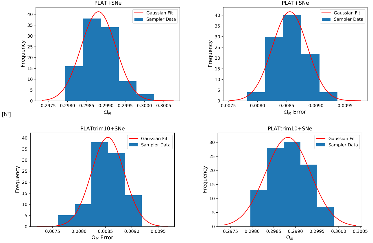
Figure A1. The two uppermost panels depict the MCMC sampler results for \Omega_M (upper left) and its error (upper right) considering PLAT+SNe Ia probes together. The bottom panels show the same considering instead PLATtrim+SNe Ia probes. The PLATtrim sample in this Figure refers the apriori trim taken of the 10 GRBs closest to the fundamental plane.
