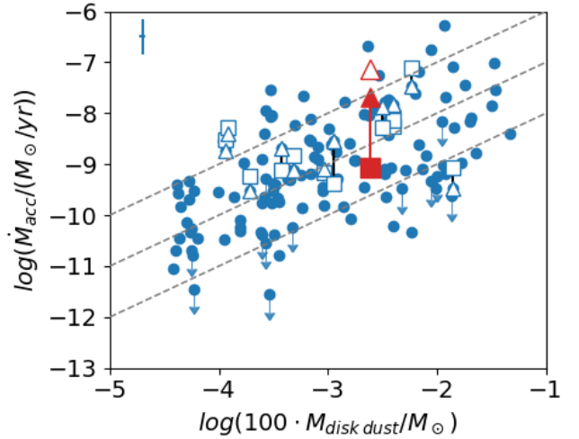
Fig. 3. Measured \dot{M}_{\text{acc}} and \dot{M}_{\text{disk}} for targets in the Lupus and Chamaeleon I star-forming regions (blue filled dots). The red filled (empty) triangle and square indicate the 2010* (2010) and 2021 mass accretion rates of XX Cha, respectively. The dashed lines display the \dot{M}_{\text{disk}}/\dot{M}_{\text{acc}} ratio of 0.1, 1, and 10 Myr, respectively. The white empty squares and triangles indicate targets observed in 2021 in the PENELLOPE program (Manara et al. 2021) and around 2010, respectively.
