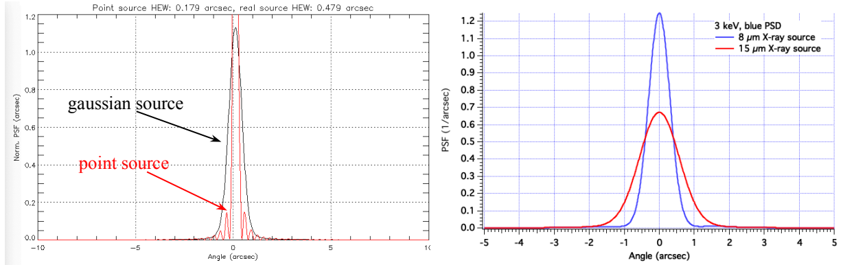
Figure 6: Left: expected PSF for a point-like source (red line) and for an 8 \mu\text{m} FWHM X-ray source (black line). Right: computed PSF at 3 keV for different FWHM values of the X-ray source.
