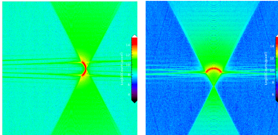
Figure 16. Left: the effect of a 20 \mu\text{m} translation of the parabolic segment in the VERT-X mirror along the x -axis on the X-ray image at 1.2 keV, as imaged on a 0.2 mm-wide detector. The color scale is logarithmic. The HEW is 0.93 arcsec.
