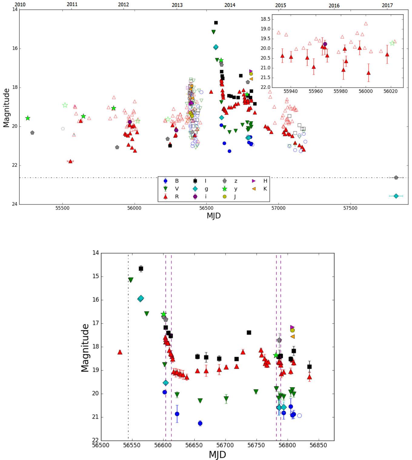
Figure 2. Optical and NIR light curves of SN 2013gc. Top: the full 7-yr coverage. For the sake of clearness, error bars are not reported here. A blow-up of the light curve of the transient during the 2012 variability period (see Section 6) is shown in the top-right inset. The horizontal line indicates the magnitude of the brightest detection of 2017, showing that the object has faded with respect to the pre-SN eruptive phase. Bottom: blow-up of the post-explosion evolution. The purple dashed lines mark the epochs of the available spectra, while the black dot-dashed line marks the date of the assumed maximum. Upper limits are indicated as empty symbols. For each band, a different symbol is used.
