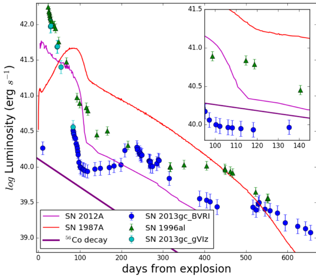
Figure 9. Quasi-bolometric BVRI light curves of SNe 1987A, 1996al, 2012A, and 2013gc. The inset shows a blow-up of the region between 95 and 145 d after the explosion, in which there is evidence of 56 Co radioactive decay. The decay slope of 56 Co [0.98 mag (100 d) -1 ] is reported with a purple line for comparison. The early-phase ( gViz ) bolometric light curve is plotted with cyan dots.
