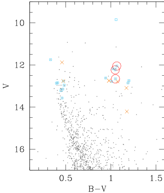
Figure 7. CMD of NGC 2355 with the three stars observed with NOT at FIES indicated by large red circles. Light blue squares indicate member stars and orange crosses non-members (from Soubiran et al. 2000; Mermilliod et al. 2008; Jacobson et al. 2011b) in common with our photometry.
