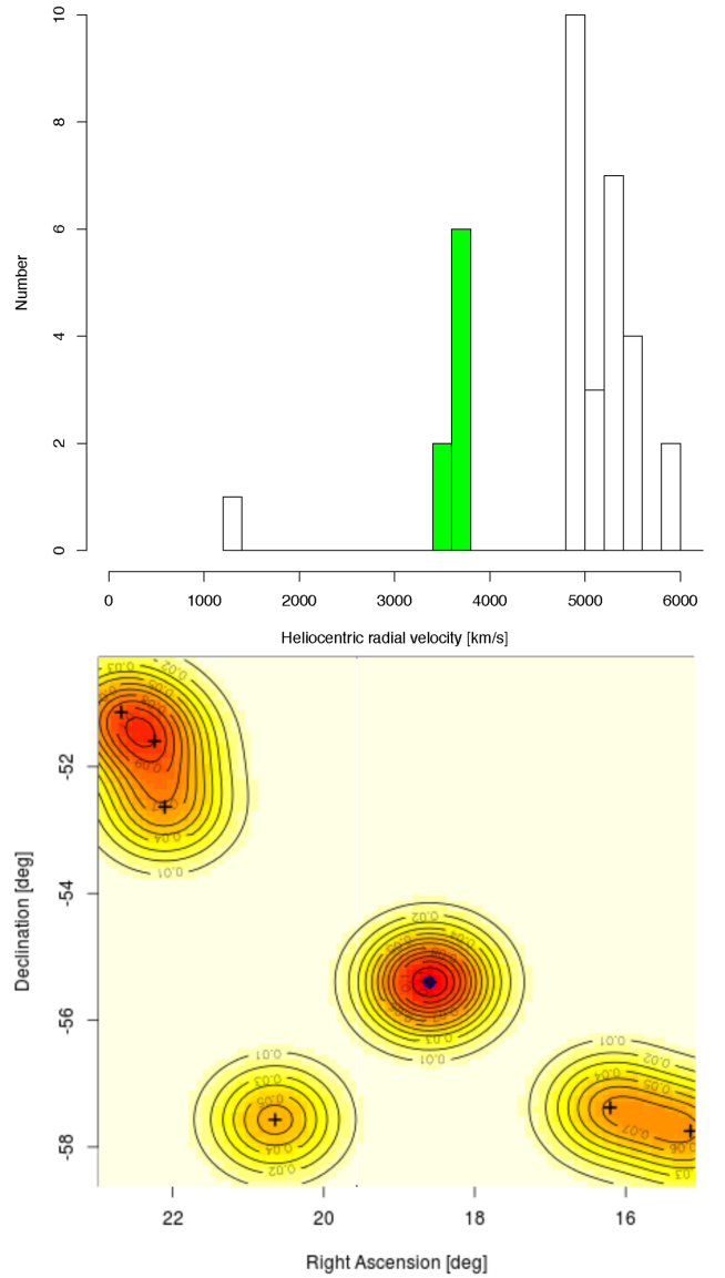
Figure A1. Top panel: histogram of the heliocentric radial velocity of galaxies within a box of 4 \times 4 \text{ Mpc}^2 in the range 1000\text{--}6000 \text{ km s}^{-1} . Bottom panel: spatial distribution of galaxies in green in the top panel, i.e. the neighbours of the NGC 454 system. The map is normalized to the total density. Galaxies in the area are listed in Table A1.
