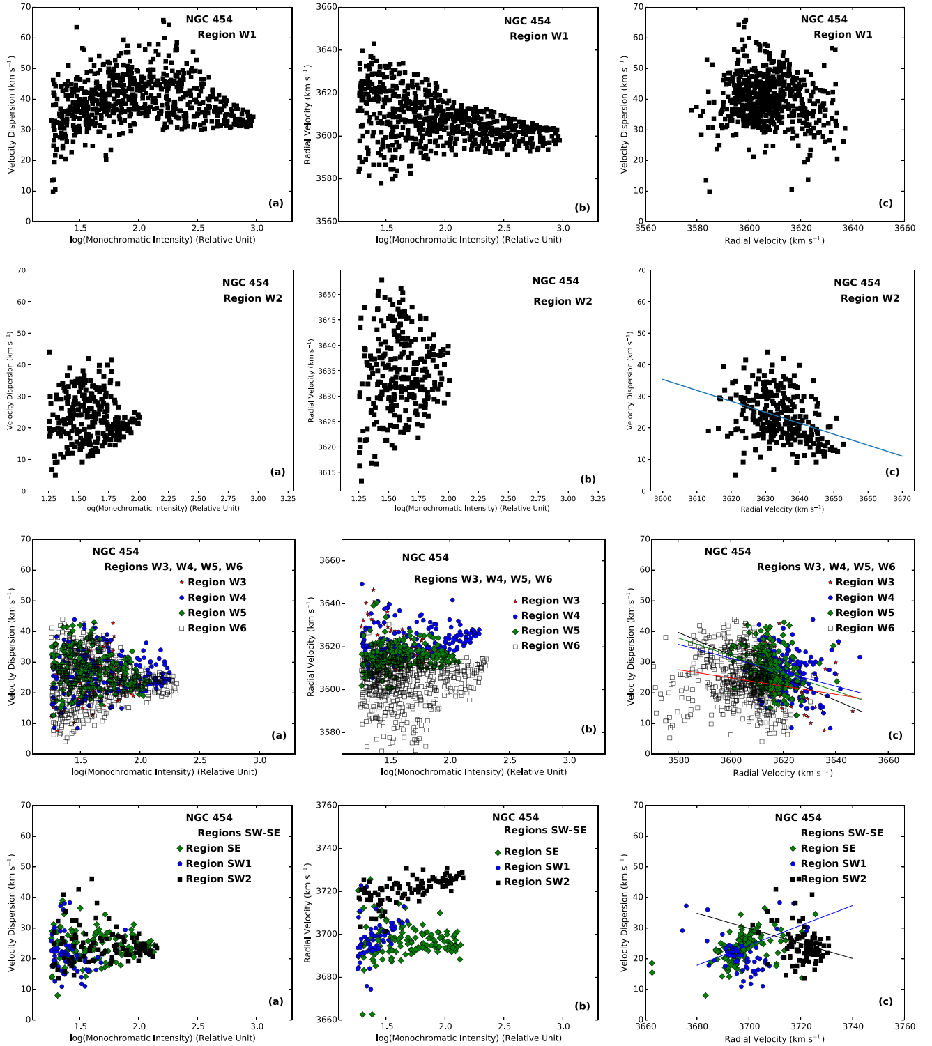
Figure 7. From top to bottom: panels (a) ( I-\sigma ), panels (b) ( I-V_r ), panels (c) ( V_{\text{hel}}-\sigma ) diagnostic diagrams in the W1–W6 complexes in NGC 454 W and in the NGC 454 SE and SW complexes. The plot results from a single Gaussian fit to the line profile. Solid lines in V_r-\sigma diagrams represent the linear regressions applied when Pearson’s correlation test is robust.
