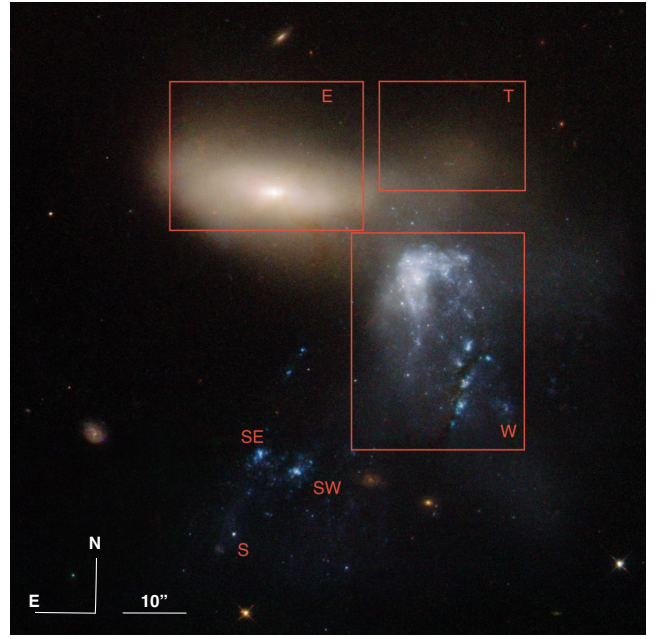
Figure 1. Colour composite image of the NGC 454 system obtained with HST -Wide Field Planetary Camera 2 in the F450W ( B ), F606W ( V ) and F814W ( I ) filter by Stiavelli et al. (1998). The figure highlights the different regions of the system following Johansson (1988) E and W areas including the early-type and the late-type member of the pair, respectively; S, SW and SE are knots likely connected to the W member. T is an area introduced by Stiavelli et al. (1998, see the text). The size of the FoV is 1.66 arcmin.
