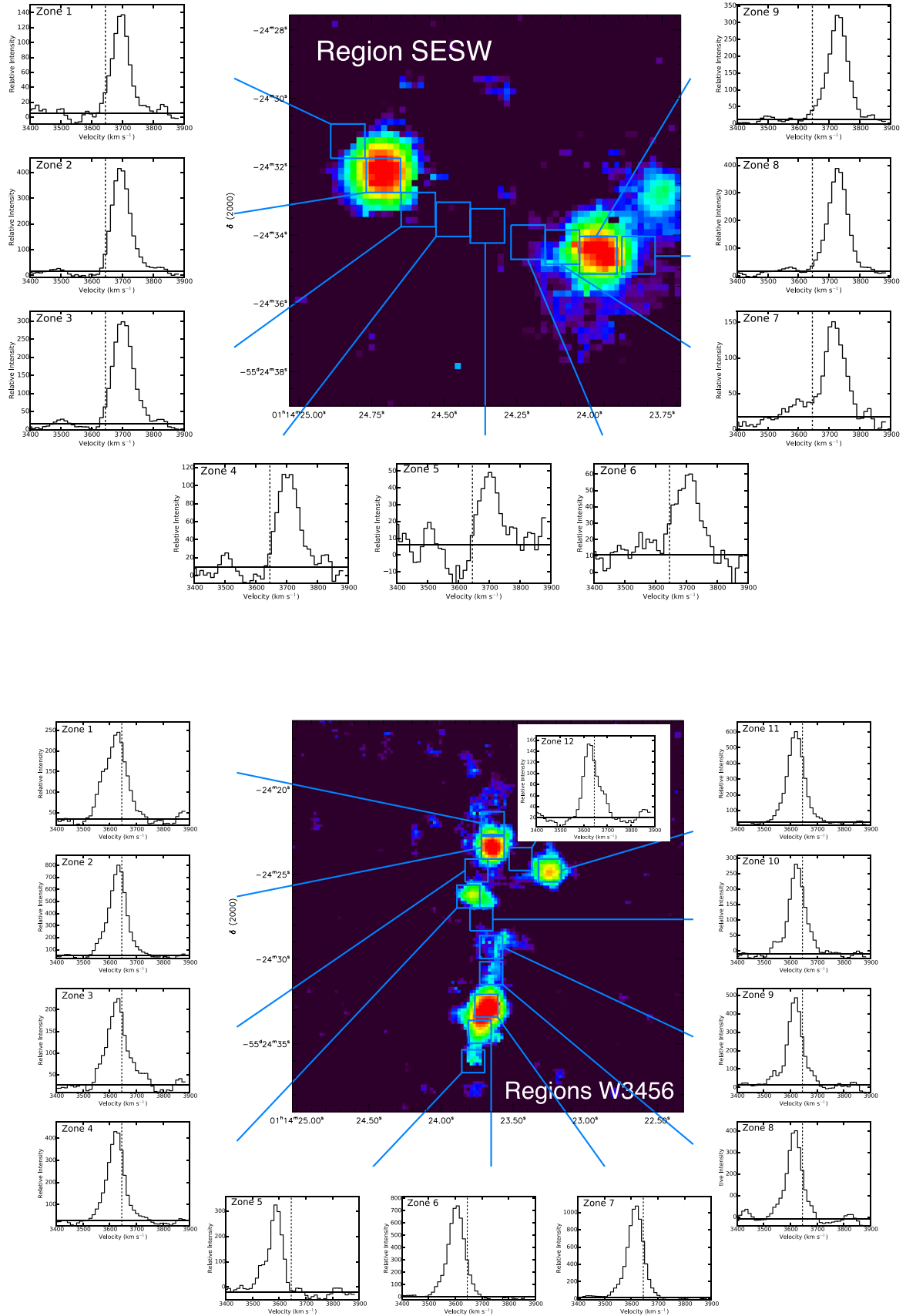
Figure 6. Emission profiles in NGC 454 SE and NGC 454 SW (top panel) and in the NGC 454 W region between the W3 and W6 complexes (bottom panel). The vertical dotted line indicates the adopted systemic velocity V_{\text{hel}} = 3645 \text{ km s}^{-1} . The horizontal line indicates the mean continuum level. The map corresponds to the monochromatic emission.
