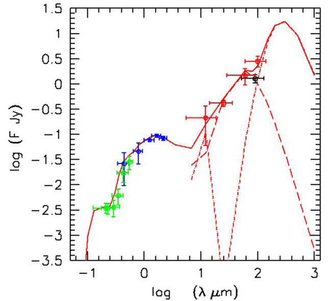
Figure 11. Observed SED of the whole NGC 454 system. The contribution of both the dust components to the FIR SED is also shown: dot-dashed and the long-dashed lines are the warm and the cold dust components, respectively (see the text). The solid line represents the resulting SED. Green symbols represent our Swift -UVOT observations and blue symbols B , R , IRAS and 2MASS J , H , K measures. Red symbols are IRAS data while the black symbol is the AKARI /FIS detection.
