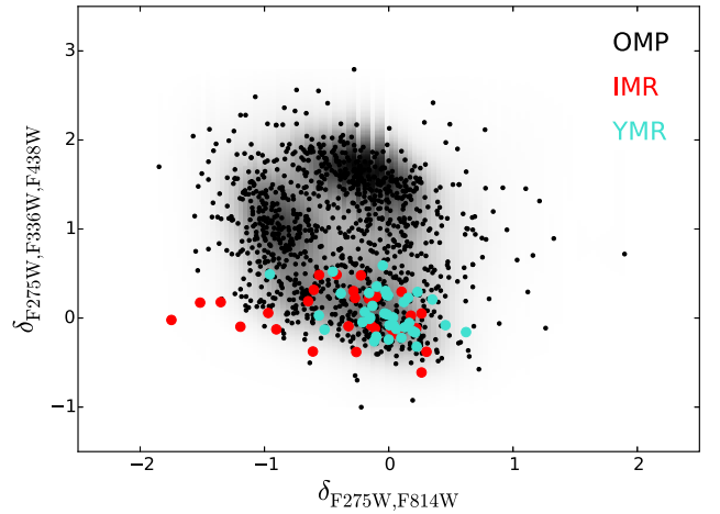
Figure 3. Metallicity-normalized chromosome map. The old, metal-poor population is shown in black and shows the clear signature of ‘multiple populations’ with three main concentrations in this diagram. The intermediate age, metal-rich population (IMR, in red) and the young, metal-rich population (YMR, in blue), however, belong only to the lower right clump, which is where stars with ‘normal’ or field composition are expected to lie.
