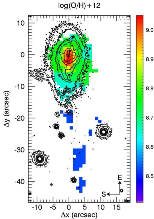
Figure 24. SOS 90630. The O/H abundance ratios derived using the PVQZ module.
