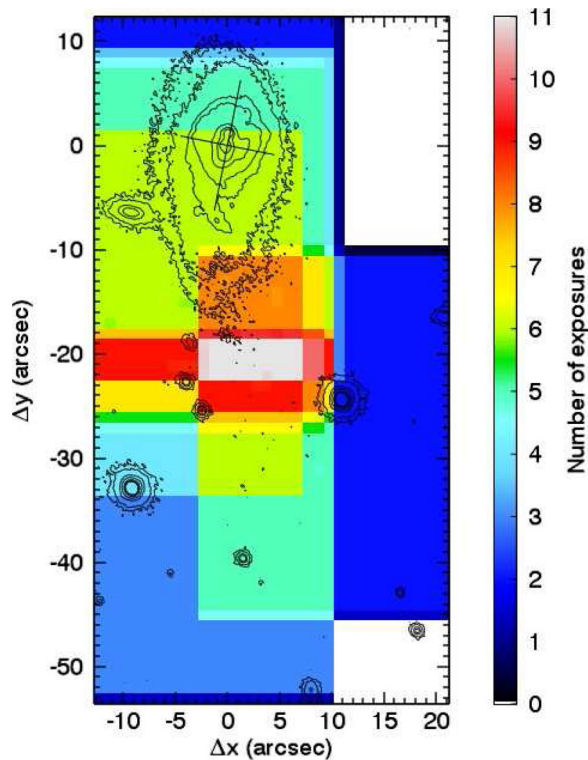
Figure 7. SOS 90630 . Same as Fig. 6 but for SOS 90630 .
