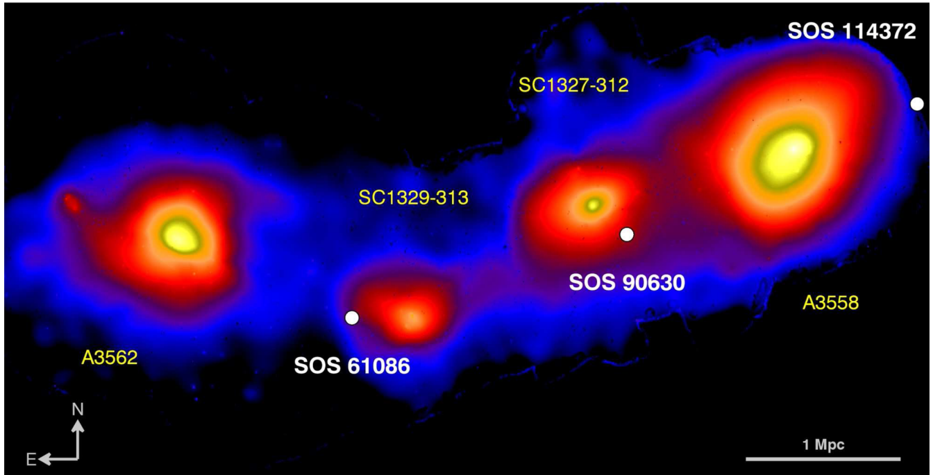
Figure 1. The positions of SOS 61086 and SOS 90630 (white dots) are indicated on the X-ray emission map including four out of five clusters of the SSCC. The position of SOS 114372 (see the text) is also marked. The X-ray surface brightness is derived from a wavelet analysis of XMM-Newton images extracted in the 0.5–2.5 keV energy band, which have been corrected for spatially variable effective exposure and background components. Scale and orientation are shown at the bottom.
