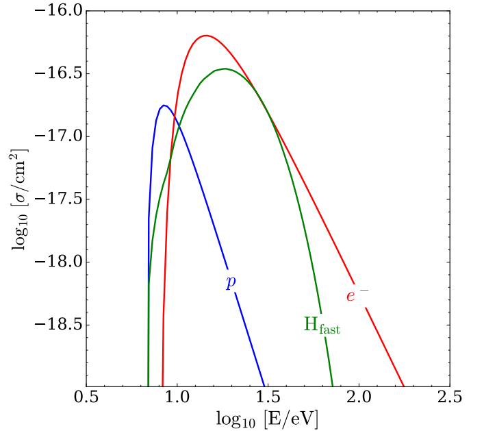
Fig. 2. The energy dependence of the dissociation cross sections by protons (blue), electrons (red), and fast hydrogen atoms (green) colliding with molecular hydrogen.
