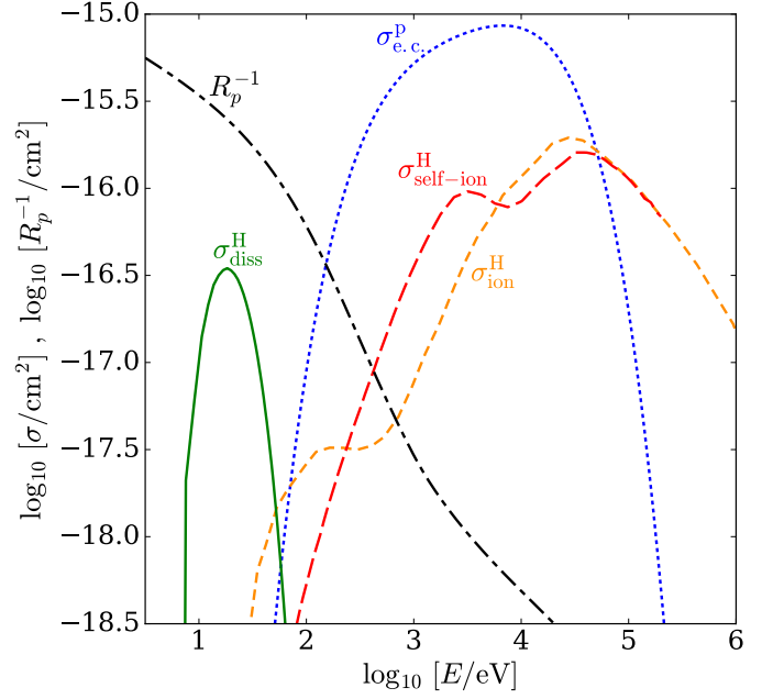
Fig. A.1. The cross sections of processes governing equilibrium distributions of protons and fast hydrogen atoms at low energies: electron capture by p (A.1, dotted blue line), ionisation of H_2 by H_{\text{fast}} (A.2, short-dashed orange line), self-ionisation of H_{\text{fast}} (A.3, long-dashed red line), and H_2 dissociation by H_{\text{fast}} (A.4, solid green line). The inverse of the proton stopping range, R_p^{-1} , is also plotted (black dot-dashed line).
