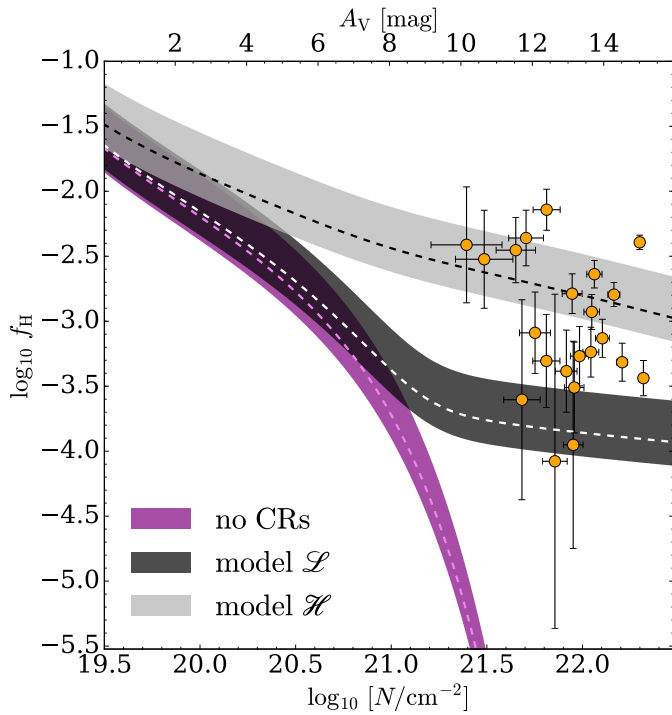
Fig. 5. Atomic hydrogen fraction versus the total column density of hydrogen (bottom scale) and visual extinction (top scale). Observations from Li & Goldsmith (2003) are shown as solid orange circles. Coloured stripes represent our results for the case of photodissociation only (purple), model \mathcal{L} (black), and \mathcal{H} (grey). Dashed lines refer to the average value of the total volume density of hydrogen (suggested by Li & Goldsmith 2003).
