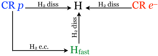
Fig. 1. Dissociation diagram showing the three main processes of production of atomic hydrogen. Labels “diss” and “e.c.” refer to dissociation and electron capture, respectively.
