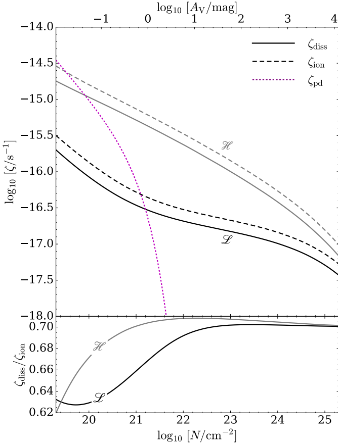
Fig. 4. Upper panel: rates of CR dissociation ( \zeta_{\text{diss}} , solid lines), CR ionisation ( \zeta_{\text{ion}} , dashed lines), and photodissociation ( \zeta_{\text{pd}} , purple dotted line) for models \mathcal{L} (black) and \mathcal{H} (grey), plotted versus the total column density of hydrogen (bottom scale) and visual extinction (top scale). Lower panel: ratio \zeta_{\text{diss}}/\zeta_{\text{ion}} for the two models.
