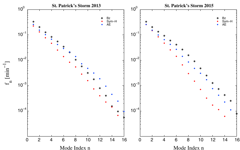
Figure 4. The characteristic frequencies, f_n , versus the mode index, n , for the IMFs relative to B_z (black star), SYM-H (red circles), and AE (blue circles). IMFs for SYM-H and AE are reported in Figures 2 and 3, respectively.
