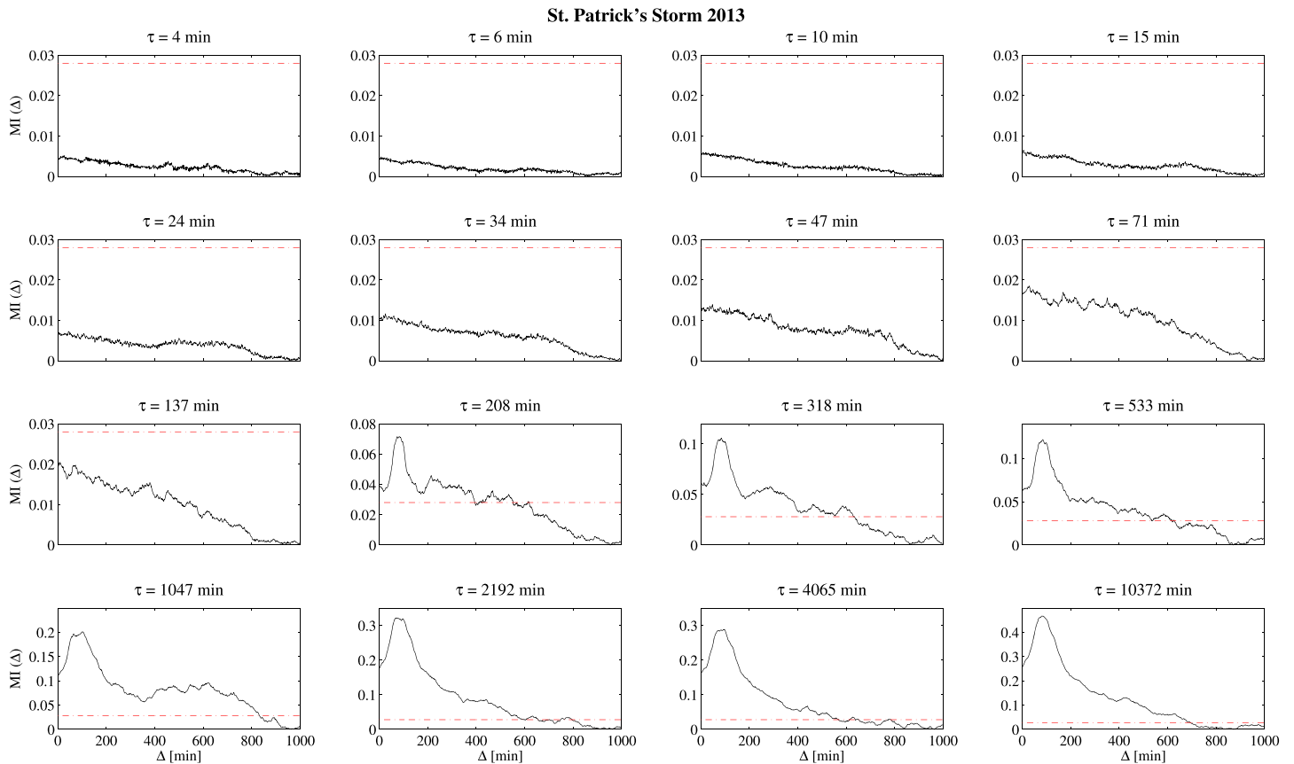
Figure 5. The scale-to-scale DMI between IMFs of the interplanetary magnetic field B_z component and auroral electrojet AE index for the St. Patrick's storm 2013 time period. Red dashed line indicates the significance (5% null hypothesis) DMI threshold, MI_{thr} = 0.028 .
