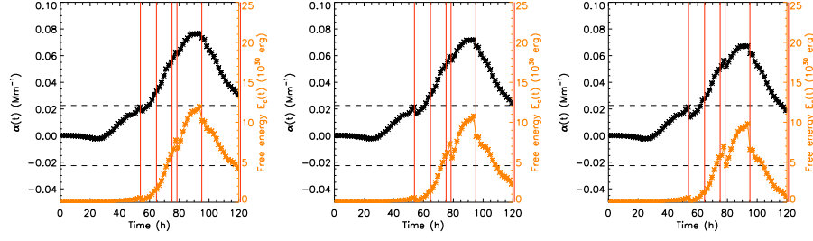
Figure 5. CME-normalized \alpha (black stars) and free energy (orange crosses), as a function of time, for the three values of the free parameter \Delta\alpha_1 = \alpha_1 \times [0.2, 0.3, 0.4] (from left to right). The horizontal dashed lines show the value of \alpha_{\max} . In all plots, the red vertical lines indicate the time of the peak of the flares (1-5) in the time series (see Table 1).
