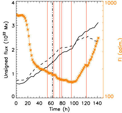
Figure 2. Time evolution of the positive (solid line) and negative (dashed line) magnetic fluxes, and of the function \mathcal{F}_l (connected asterisks) in Equations (2) and (3). The red vertical lines indicate the peak times of the flares in our time series (see Table 1), while the vertical dot-dashed line indicates the time of the central meridian passage of the AR. Time starts at 00:00 UT on 24 May 2003.
