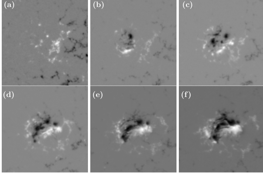
Figure 1. From left to right and from top to bottom, MDI magnetograms showing the magnetic configuration of AR NOAA 10365 at t=5, 25, 50, 75, 100 , and 120 h counted from 24 May 2003, 00:00 UT. North is at the top, west is on the right.
