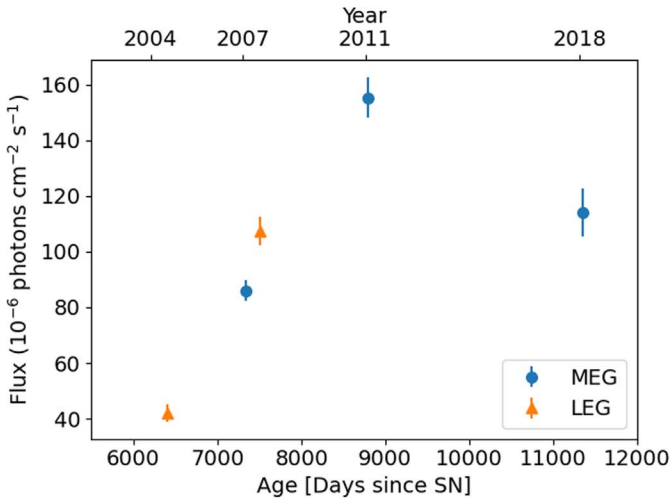
(e) Ne (Ly \alpha )
