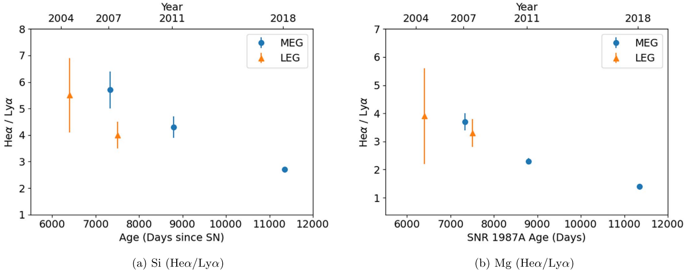
Figure 5. Temporal changes of Heα/Lyα line-flux ratios for (a) Si (Si XIII / Si XIV) and (b) Mg (Mg XI / Mg XII) based on high-resolution Chandra grating spectra of SNR 1987A.
