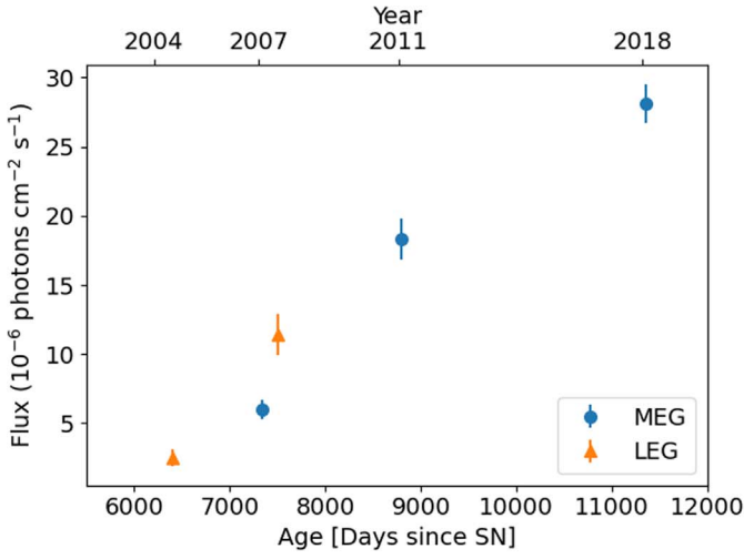
(a) Si (Ly \alpha )
