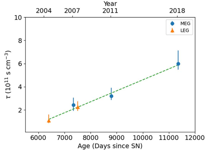
(b) Ionization Age: Hard Shock Component
