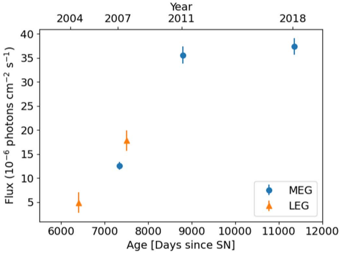
(c) Mg (Ly \alpha )
