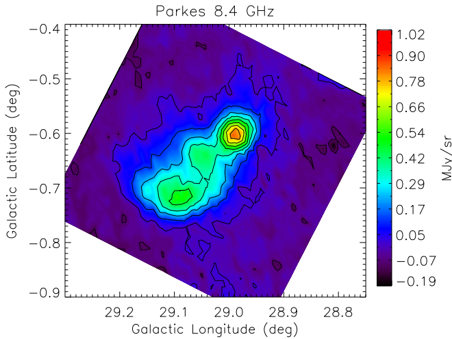
Figure 1. 8.4 GHz map of RCW175 obtained with the Parkes radio telescope using the MARS receiver. The angular resolution is 2.4 arcmin FWHM and sensitivity is 22 mJy beam -1 . The contour intervals are 10% of the peak emission.
