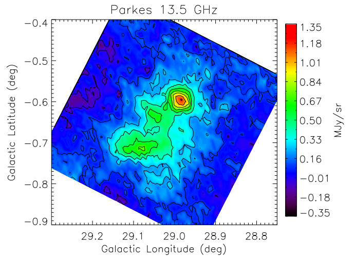
Figure 2. 13.5 GHz map of RCW175 obtained with the Parkes radio telescope using the Ku-band receiver. The angular resolution is 1.7 arcmin FWHM and sensitivity is 18 mJy beam -1 . Contours show levels each ranging 10% of the peak emission.
