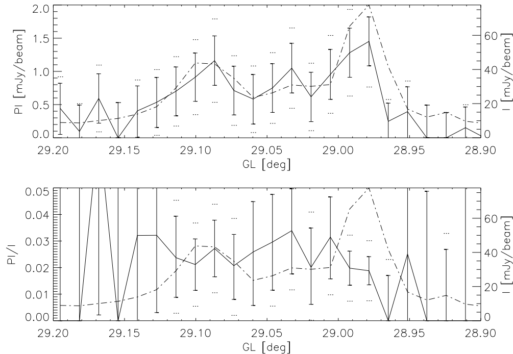
Figure 10. Linear polarization measurements performed at 21.5 GHz. For polarization measurements, one-dimensional scans have been performed on RCW175 with coordinates shown in Figure 4. The top panel displays the polarized intensity (solid line) along with an indication of the emitted intensity in arbitrary units (dot-dashed line). The error bars on PI show 2\sigma statistical uncertainties (solid line). The dotted bars show the linearly summed statistical uncertainties ( 2\sigma ) to twice the systematic uncertainty (i.e., 2 \times 11\% ). In the bottom panel we show, with a solid line, the relative polarized emission and, with the dot-dashed line we give an indication of the intensity emitted at 21.5 GHz. Also in this plot we include 2\sigma statistical uncertainties arising from PI and I measurements and in the dotted bars we linearly added to the 2\sigma statistical uncertainty, twice the residual instrumental polarization we qualified with 0.3%. Measurements are one beam spaced.
