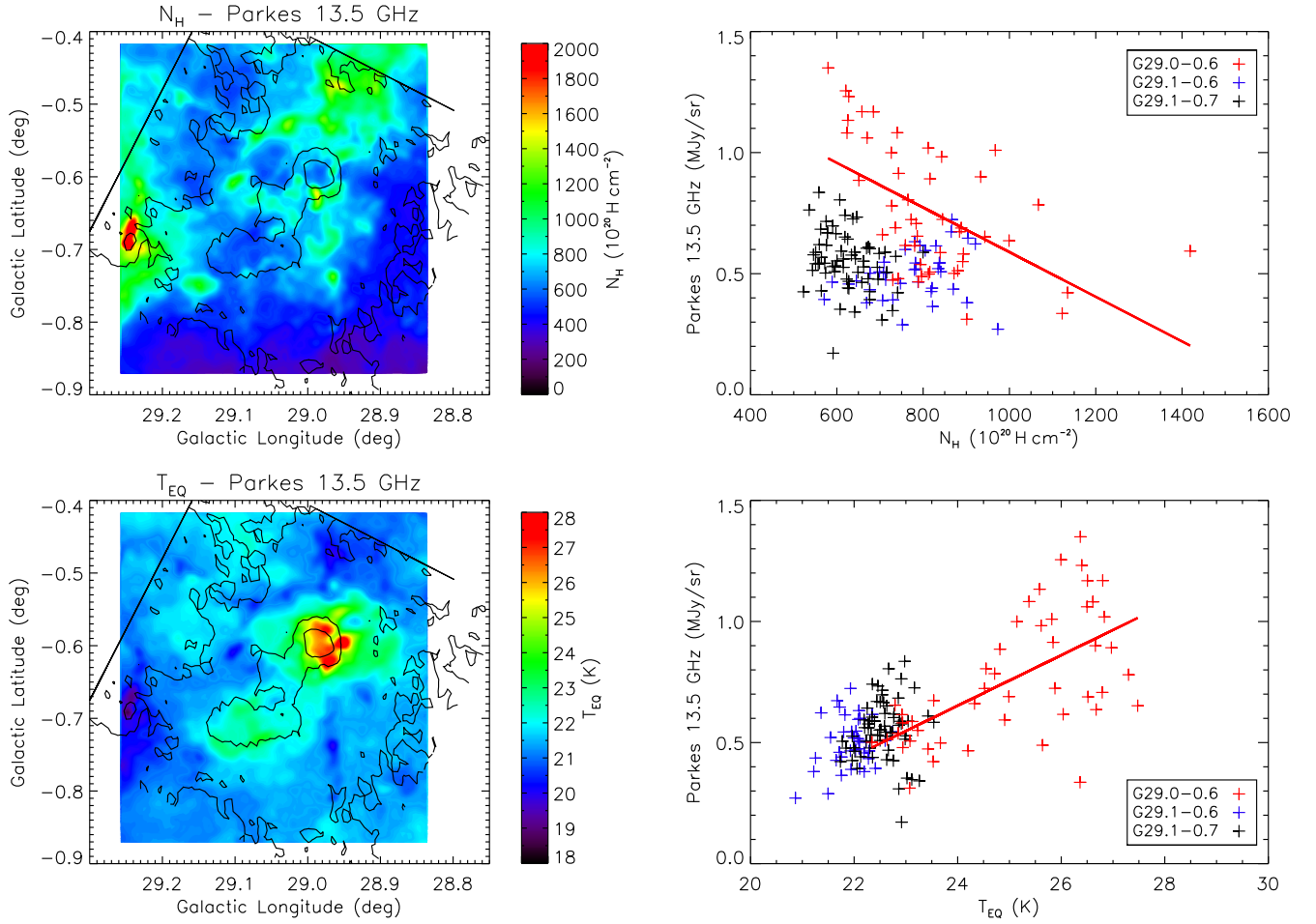
Figure 9. Ku -band 13.5 GHz map vs. DUSTEM N_H and T_{EQ} maps (top to bottom). The DUSTEM parameter maps, with the 13.5 GHz in contours (with levels at 0%, 33%, and 66% of the peak values), are shown on the left. The corresponding scatter plots, i.e., microwave map vs. parameter map, are shown on the right. Different colors identify different regions, following the color scheme in Figure 4.
