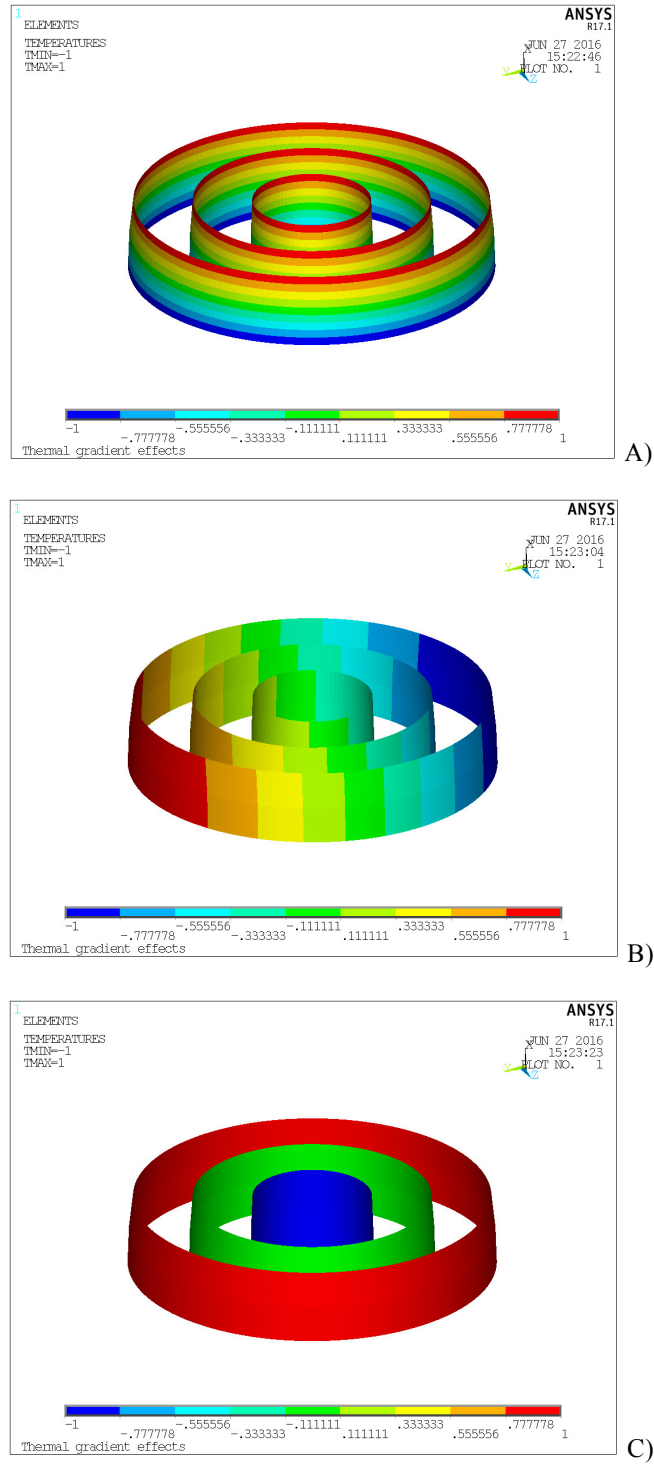
Fig. 2. Thermal Gradients considered for the preliminary study ; A) T1 – Axial temperature gradients \pm 1K ( \sigma_{MAX} cold), B) Lateral temperature gradient ( \pm 1K ) ; C) Radial temperature gradient ( \pm 1K )
