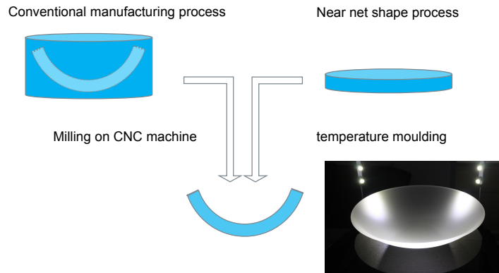
Fig. 5. Scheme of the near-net-shape process based on thermal slumping already under study at Heraeus Quarzglas GmbH & Co KG. A pseudo-spherical substrate developed in this way it is also shown (courtesy of Heraeus Quarzglas GmbH & Co KG).
