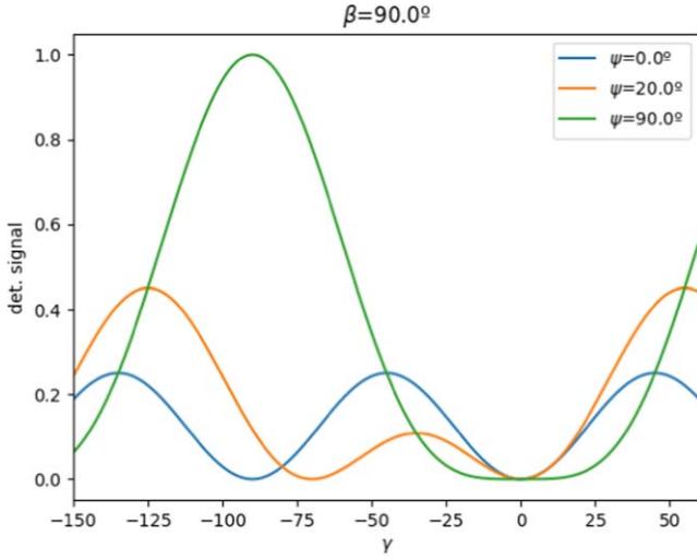
Figure 11. Model signal derived through Mueller formalism for three different configurations of the COSMOCAL's polarizer (P1), as a function of \gamma , corresponding to the rotating polarizer (P2).
