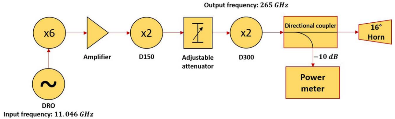
Figure 2. COSMOCal radio-frequency chain scheme.
