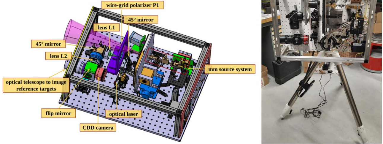
Figure 1. Left: mechanical drawings of the COSMOCal box containing the: microwave source components (right) and the optical system (left). Right: first assembled version.
