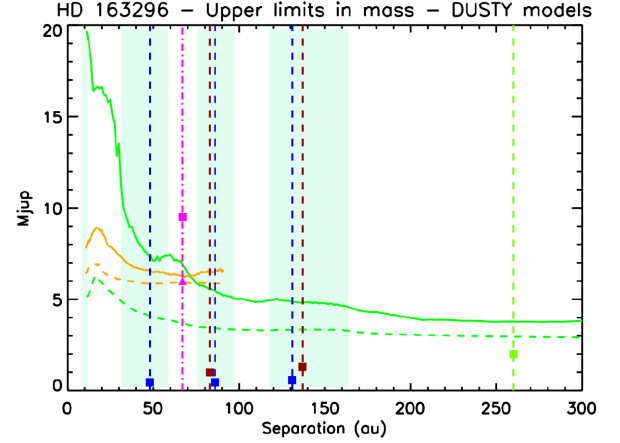
Figure 5. Same than Fig. 4 but for mass limits obtained using DUSTY models.
