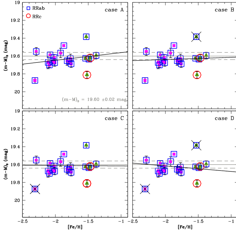
Figure 11. Distance moduli for the 20 RRL in our DZ sample as a function of [\text{Fe}/\text{H}] (spectroscopic metallicities from C05). The solid grey line is the distance modulus \pm 2\sigma (dashed lines) estimated using as a reference the PL relation derived by Neeley et al. (2017) and only the RRAb stars in the D4 sample. Metal-poor sources are magenta squares and metal-rich are green triangles. RRAb and RRc stars are encircled by blue squares and red circles respectively. The RRL marked with a cross are the rejected stars. The least squares fit (black line) has been calculated in four different cases: considering the whole sample (case A, top-left panel), removing the “closest” star (in terms of distance from us; top-right panel, case B), removing the “most distant” star (case C, bottom-left panel) and excluding both (case D, bottom-right panel). In every case the slope ( d\mu/d[\text{Fe}/\text{H}] ) is consistent with zero within 1\sigma (see text and Table 8 for details).
