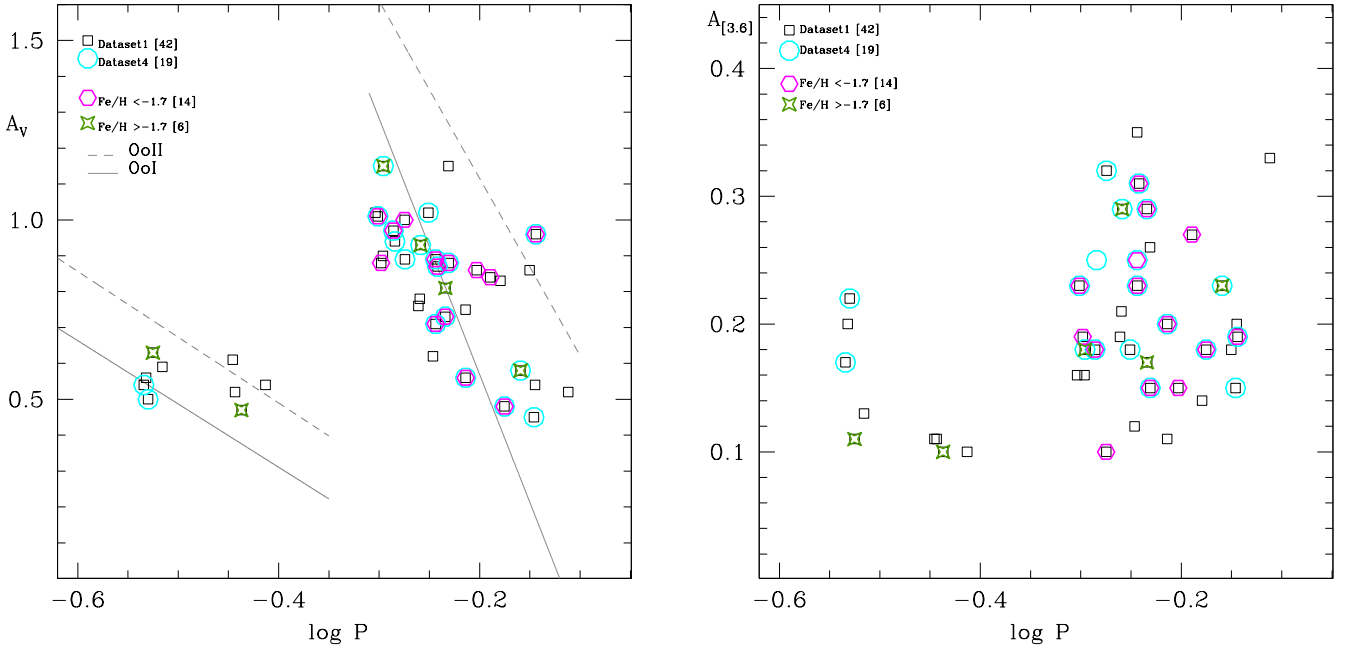
Figure 10. Left: V-band period-amplitude diagram for the 42 RR Lyrae stars of Sculptor, periods and amplitudes are from K95 and C05. The grey lines mark the loci of the OoI (solid) and OoII (dashed) Galactic GCs from Clement & Rowe (2000) where, typically, OoI systems are more metal-rich ( [\text{Fe}/\text{H}] \sim -1.5 dex) than the OoII systems ( [\text{Fe}/\text{H}] \sim -2 dex). Black empty squares are the D1 sample while cyan circles are the D4 sample. Magenta hexagons and green four-pointed stars denote metal-poor and metal-rich samples, according to C05 metallicities. Right: Mid-infrared period-amplitude diagram, adopting the amplitudes at 3.6 \mu\text{m} derived in this study. Colours and symbols as on the left panel.
