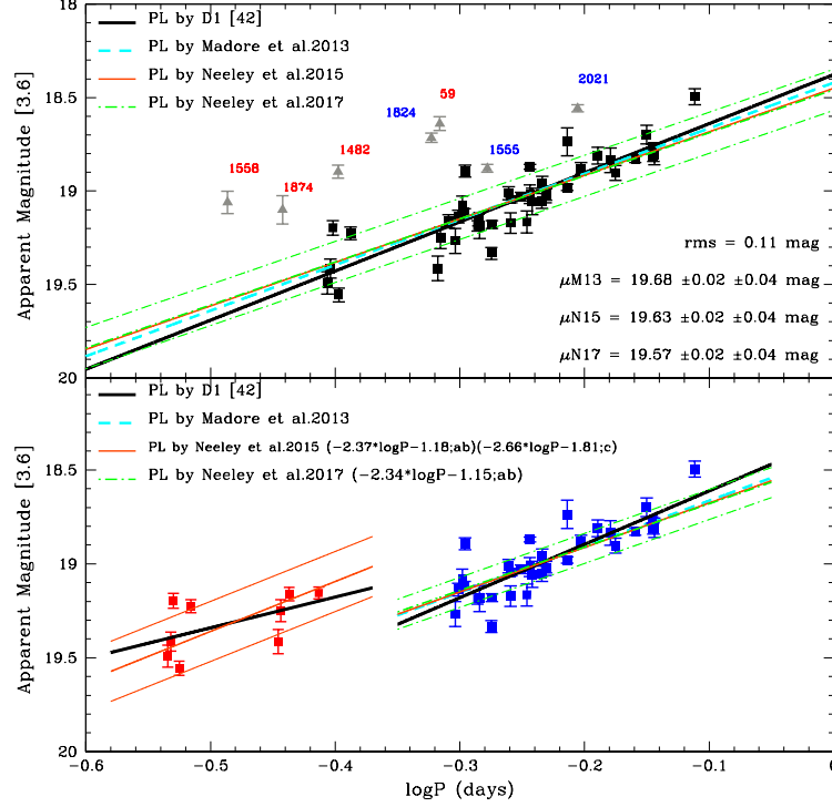
Figure 4. Top: 3.6 \mu\text{m} Period-Luminosity relations defined by the 42 RR Lyrae stars observed in Sculptor (D1 sample). The periods of the RRC stars have been fundamentalised. The black solid line represents the least squares fit to the data in Table 1. The triangles are the most problematic stars not used in the least square fit. Bottom: RRab (blue symbols) and RRC (red symbols) stars are plotted in two PL relations that were computed from the fundamental-mode and the first-overtone pulsators separately. In both panels the cyan (dashed), orange (thin solid) and green (dash-dot) lines mark Madore et al. (2013), Neeley et al. (2015) and Neeley et al. (2017) PL relations respectively. We show only \pm 2\sigma the deviation lines of the Neeley et al. (2017)’s PL, the dispersions of the other PL relations are similar or slightly broader.
