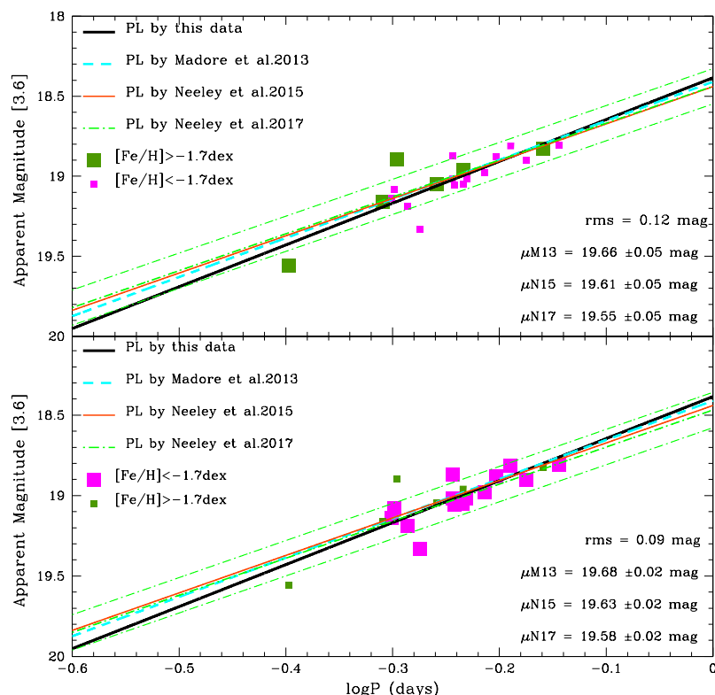
Figure 8. PL relations for the only 20 RRL (DZ sample) whose spectroscopic metallicities are known from C05. Green and magenta filled squares mark metal-rich and metal-poor RRL, respectively. The black solid line represents the least squares fit to the metal-rich (top panel) and metal-poor stars (bottom panel), respectively. The green (dash-dot) lines indicate the Neeley et al. (2017) PL relation \pm 2\sigma deviation. Similarly, the cyan (dashed) and orange (thin solid) lines mark the Madore et al. (2013) and the Neeley et al. (2015) PL relations along with their \pm 2\sigma deviations. The periods of the RRL stars have been fundamentalised .
