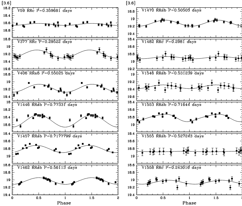
Figure 2. Light curves in the [3.6]-band for our sample of 49 RR Lyrae stars in the Sculptor galaxy. The stars are ordered with increasing ID number adopting the nomenclature from K95 and C05. The solid black lines represent the light curve models generated by GRATIS using all phase-points. V59, V1482, V1555 and V1558 are problematic stars not used to fit the PL relations (see Sect. 3.1 and Table 1). The first 12 light curves are shown here, the remaining are plotted in Appendix A.
