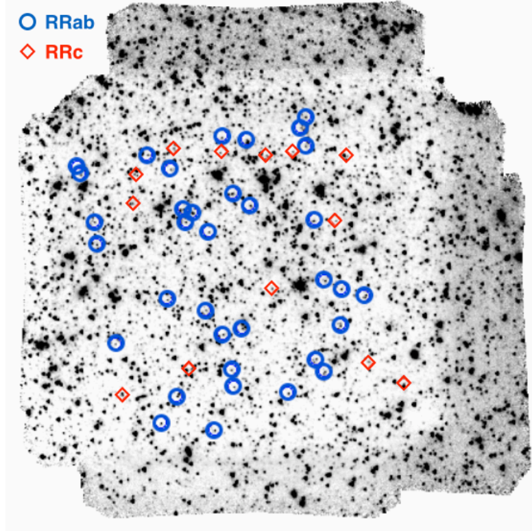
Figure 1. IRAC- Spitzer master mosaic at 3.6\ \mu\text{m} that shows the 49 Sculptor RR Lyrae stars in our sample encircled by blue open circles (RRab stars) or red diamonds (RRc stars). The field of view of the IRAC frame is 5' \times 5' . North is up and east is to the left.
