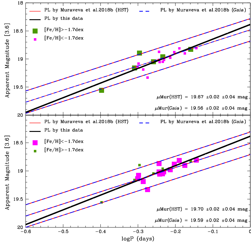
Figure 9. Same as in Figure 8 but with the thick solid red and the dashed blue lines showing the PL relations by Muraveva et al. (2018b), calibrated respectively on the HST and Gaia parallaxes, \pm 2\sigma deviation. The periods of the RRc stars have been fundamentalised .
