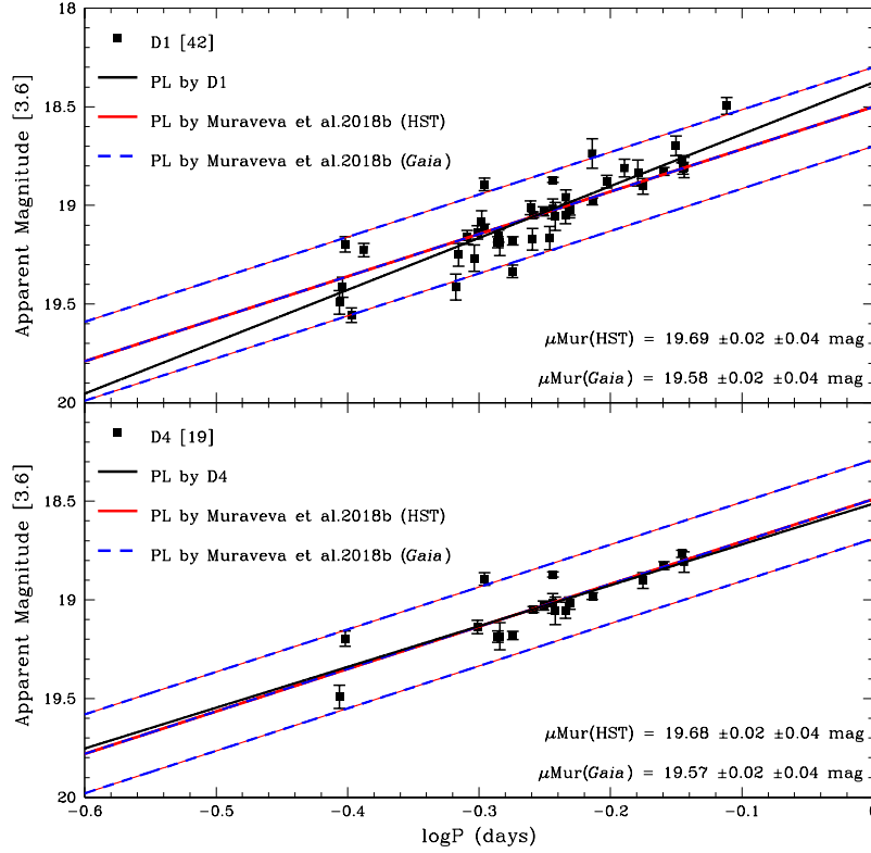
Figure 6. 3.6\ \mu\text{m} Period-Luminosity relations defined by RRab+RRc stars in the D1 and D4 samples (black solid lines), compared with the PL relations by Muraveva et al. (2018b) calibrated on HST and Gaia parallaxes (thick solid red and dashed blue lines respectively). The periods of the RRC stars have been fundamentalised .
