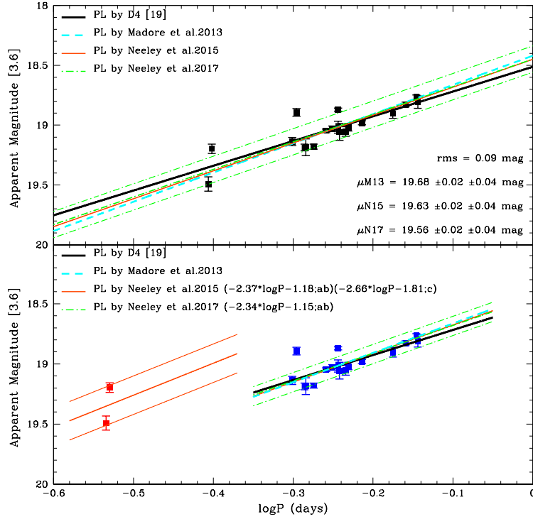
Figure 5. 3.6 \mu\text{m} Period-Luminosity relations defined by the 19 RR Lyrae stars that compose the D4 sample. Symbols, colours and \pm 2\sigma dispersion lines are as in Figure 4.
