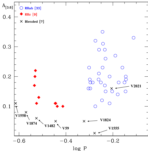
Figure 3. Mid-infrared period-amplitude diagram for all the RRL in our sample based on light curves at 3.6\ \mu\text{m} . The blue open circles and the red diamonds mark the RRab and RRe stars respectively. The RRL affected by crowding/blending and discarded in this study are labelled and marked with crosses.
