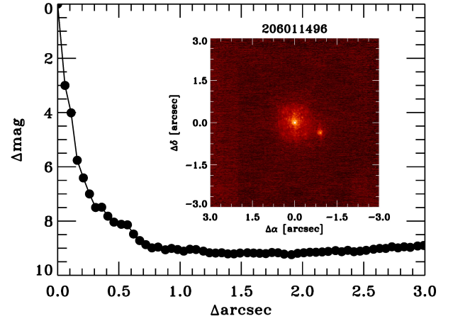
Fig. A.1. K-band Keck AO image shows a companion at a separation of \approx 979 \pm 5 mas.
