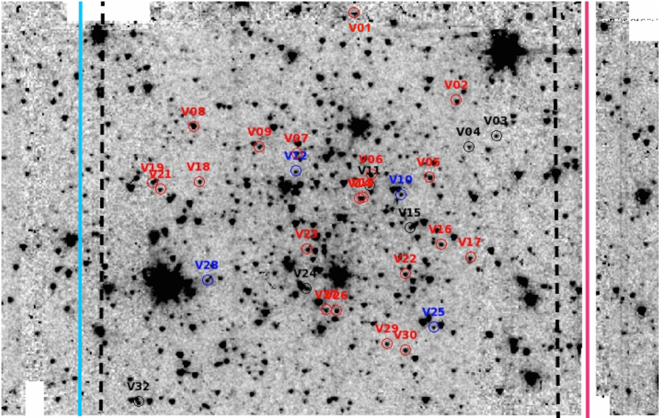
Figure 4. Zoom-in of Fig. 1 showing the region of the Reticulum cluster. Open red, blue, and black circles indicate the Reticulum RRetab, RRetc, and RRetd stars, respectively.
