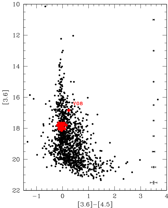
Figure 2. CMD ([3.6] versus [3.6]−[4.5]) of 1284 sources in the field of Reticulum observed with Spitzer in both 3.6 and 4.5 \mu\text{m} passbands. RRLs are marked in red. Typical uncertainties of the photometry per magnitude bin estimated with ALLFRAME are shown on the right.
