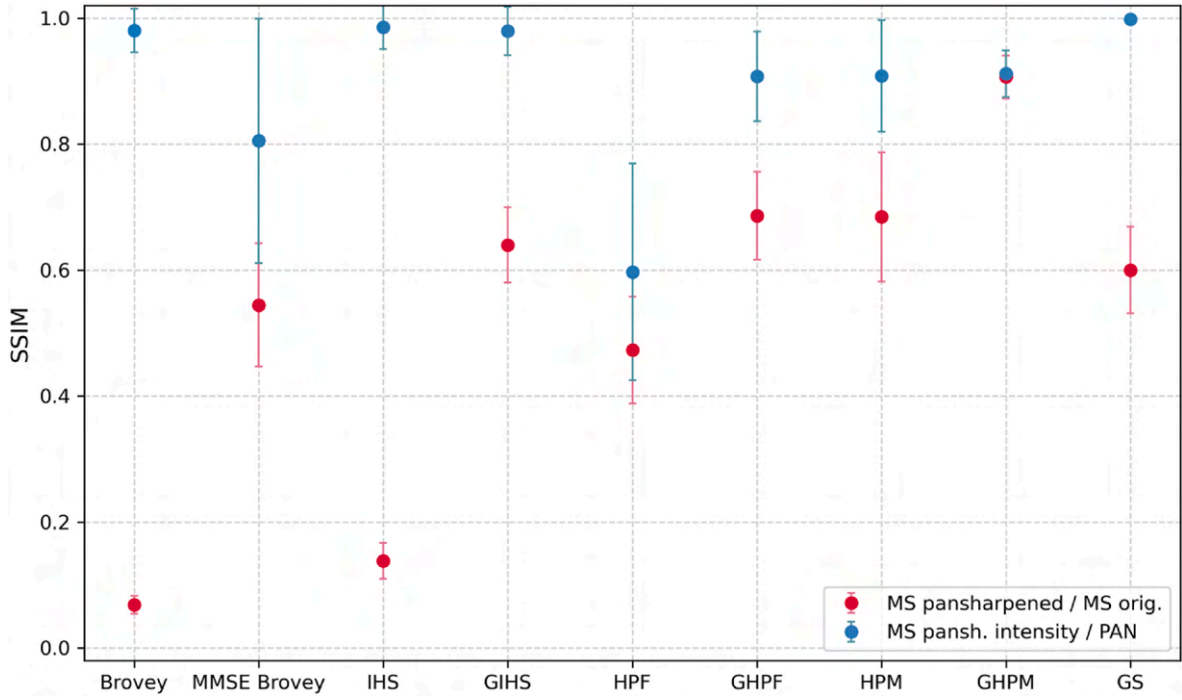
Fig. 6. Comparison of averaged Structural Similarity Image Measure (SSIM) parameters derived from the comparison of the results with the pre-transformation CaSSIS image at RR in red, and with the reference RED HiRISE at FR in blue, listed by method. The parameter analyses the structural properties of the images, whereby the discrepancy between the two values reflects the gain in visual details that ideally match the panchromatic, and the deviation from the original image. The error bars indicate the measured standard deviation for the dataset.
