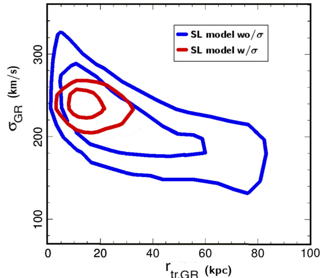
Figure 6. Probability contours of the GR velocity dispersions versus the truncation radius from the MCMC sampling for the model ‘wo/ \sigma ’ (in blue) and ‘w/ \sigma ’ (in red). The knowledge of the galaxies velocity dispersions improves the constraint on the global scaling relation, tightening the constraints on the galaxy truncation radii by \sim 50 per cent.
