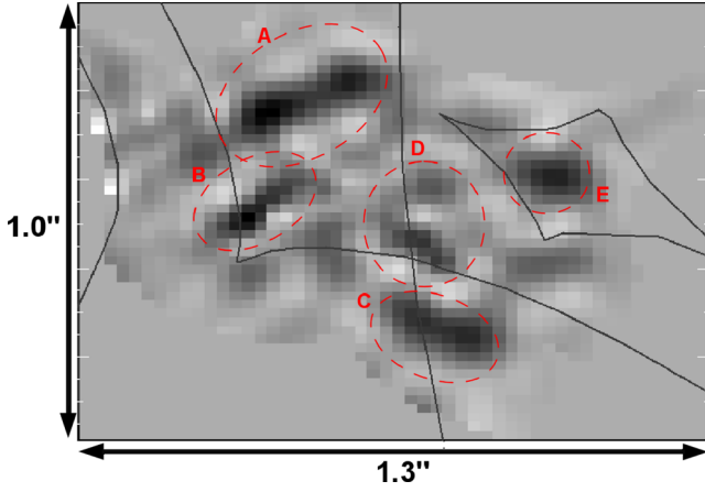
Figure 10. Source reconstruction of the southern arc (1.3 arcsec \times 1.0 arcsec cutout, which corresponds to \sim 10 \text{ kpc} \times 8 \text{ kpc} at the redshift of the source). The grey lines are the caustics. The reconstructed source is composed of five clumps (red dashed contours). The clumps A–B corresponds to the system 3 in the point-like models, while C–D–E are the light reconstruction of system 4.
