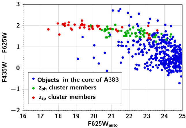
Figure 3. Colour-magnitude diagram for the sources extracted in the core of A383. We plot the colour from aperture magnitudes in the filters F435W and F625W versus the SExtractor \text{mag\_auto} in the F625W filter. Blue circles are all the sources extracted in the cluster core; in red we plot the spectroscopically confirmed cluster members and in green the photometric cluster member candidates with z_{\text{ph}} \in [0.16, 0.22] .
