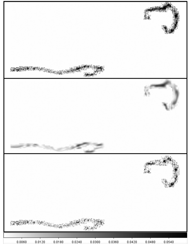
Figure 9. Surface brightness reconstruction of the giant southern arcs (20 arcsec \times 10 arcsec cutout, which corresponds to \sim 60 \text{ kpc} \times 30 \text{ kpc} at the cluster redshift). Upper panel show the arcs in the HST/ACS/F775W filter, the central panel shows the reconstruction of the arc in this filter, and the lower panel shows the residuals.
