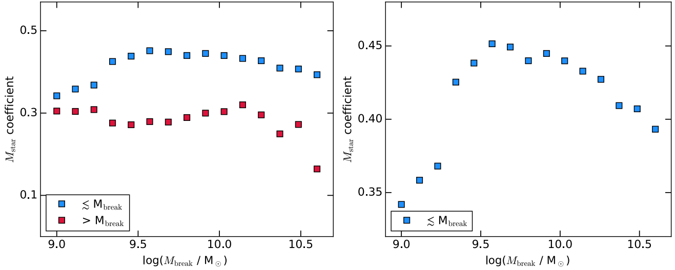
Fig. 7. PCA coefficients for MAGMA \log(M_{\text{star}}) plotted against M_{\text{break}} for the division into the two PCAs. Right panel: magnification of the left panel, showing, more effectively, that the range of M_{\text{star}} coefficients as the M_{\text{break}} mass is varied. The lower values of the M_{\text{star}} coefficient toward higher M_{\text{break}} results from the flattening of the MZR at high M_{\text{star}} .
