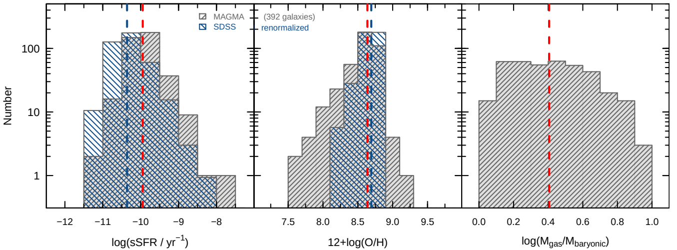
Fig. 3. Distributions for combined sample of 392 galaxies for \log(\text{sSFR}) ( left panel ), 12 + \log(\text{O}/\text{H}) ( middle ), and \log[M_{\text{gas}}/(M_{\text{star}} + M_{\text{gas}})] \equiv \log(M_{\text{gas}}/M_{\text{baryonic}}) ( right ). The red vertical dashed lines in each panel correspond to the MAGMA medians: \log(\text{sSFR}/\text{yr}^{-1}) = -9.92 ; 12 + \log(\text{O}/\text{H}) = 8.64 ( Z_{\odot} would be 12 + \log(\text{O}/\text{H}) = 8.69 , see Asplund et al. 2009 ); and \log(M_{\text{gas}}/M_{\text{baryonic}}) = \log(f_{\text{baryonic}}) = 0.39 . The left and middle panels also include the SDSS10 sample, as in Fig. 2; the sSFR and O/H medians of SDSS10 are \log(\text{sSFR}/\text{yr}^{-1}) = -10.36 and 12 + \log(\text{O}/\text{H}) = 8.69 , respectively, and they are shown by blue vertical dashed lines.
