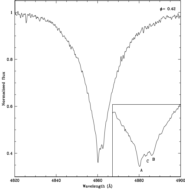
Fig. 6. Composite H_\beta of HD 216494. The contribution of the third companion is clearly visible.
