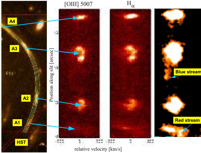
Fig. 26. Left panel: Curved slit used for the LUCI-ARGOS observation of the SDSS1038+4849 (SMILE) arc at z = 2.197 on an HST infrared image that covers the multiple images of the same galaxy (A2, A3, and A4) and of the companion galaxy A1. Middle panels: 2D spectra ( t_{\text{int}} = 4 h) of the [O III] \lambda 5007 line at 0.55'' resolution and of the H\alpha line ( t_{\text{int}} = 4 h) at 0.35'' resolution. Right panel: Smoothed [O III] \lambda 5007 2D spectrum to enhance the blue and the red streams.
