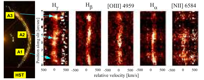
Fig. 24. Left panel: curved slit used for the LUCI-ARGOS observations on a HST infrared image of the 8 o'clock arc covering the three multiple lensed images of the galaxy at z = 2.73 . Right panel: 2D spectra of all lines observed in the H and K bands at 55\text{ km s}^{-1} spectral resolution. The integration times and spatial resolution of each band are t_{\text{int}}(K) = 2\text{ h} , \text{PSF}(K) = 0.35'' and t_{\text{int}}(H) = 3.9\text{ h} , \text{PSF}(H) = 0.35'' .
