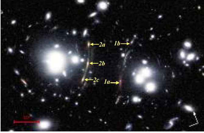
Fig. 22. Colour composite image for the central region of the massive lensing cluster G165, using LBT/ARGOS K -band for the 2016 Dec 15 run (red), + HST/WFC3 F160W (green), and F110W (blue) data. In total, 11 arclet families are discovered in this field as a result of the combined HST + K -band analysis, demonstrating the value of LUCI-ARGOS to provide high-resolution imaging that enables side-by-side comparisons (Frye et al. 2018). In addition to detecting the spatially resolved giant arc “1a” with its high estimated magnification factor of \sim 30 , the K -band data also unveil another image of this same background galaxy “1b”, that falls at its model predicted location. The secure identification of this doubly-imaged family enables us to construct a robust lens model. The brightest objects in our K image belong to the triply-imaged Arcs 2a, 2b and 2c, as labeled. North is in the direction of the compass arrow and east is to the left. A 10'' scale bar is shown in the bottom left corner for reference.
