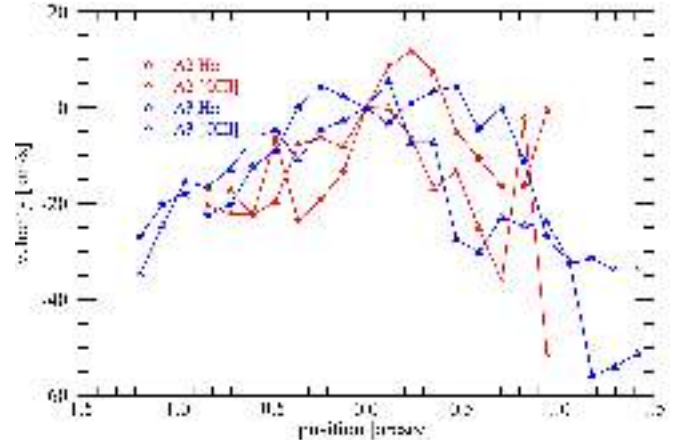
Fig. 27. Kinematics of the two images A3 (blue) and A2 (red, reversed) in SDSS 1038+4849 derived from the H\alpha observations (stars) and from the [O III] \lambda 5007 observations (triangles). The resulting curves of A2 and A3 have the typical reversed U shape of interacting systems, suggesting that the A2 and A3 images are composed of at least three clumps that are interacting with each other.
