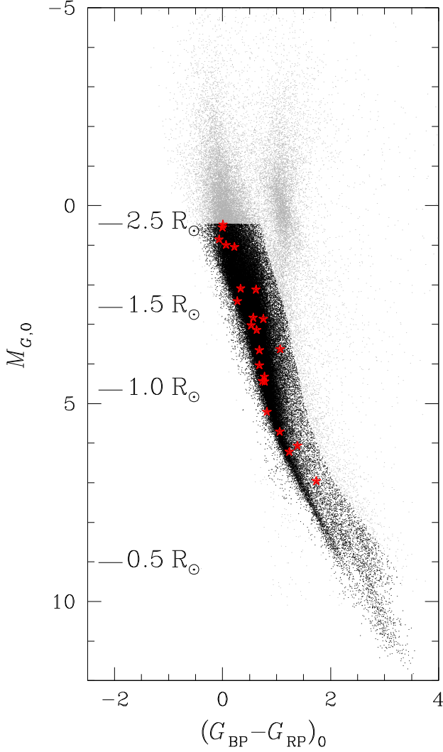
Figure 5. The M_{G,0} versus (G_{BP} - G_{RP})_0 CMD of all the stars analysed in Paper II and in this work. Black points are the main-sequence stars with R_* \leq 2.5 R_\odot , and grey points are the stars excluded from the analysis of candidate exoplanets’ frequency (see the text for details). For clarity, only 50 per cent of the stars are plotted. Red starred symbols indicate the positions on the CMD of the 23 candidate transiting exoplanets identified in stellar clusters from TESS data.
