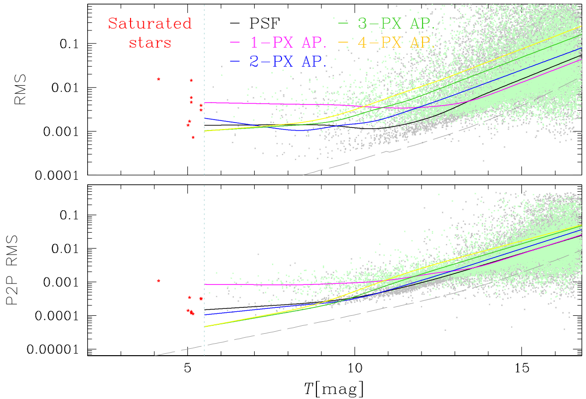
Figure 2. Mean trends of the photometric rms (top-panel) and P2P rms (bottom panel) as a function of the TESS magnitude T for different photometric methods: Black lines are associated with PSF-fitting photometry, and magenta, blue, green, and yellow lines are associated with 1-, 2-, 3-, and 4-pixel aperture photometries, respectively. As an example, the rms distributions obtained with 3-pixel and PSF-fitting photometry are shown in light green and grey crosses, respectively (for clarity, only 10 per cent of the stars are plotted). Red starred symbols represent the saturated stars. The dashed line is the theoretical limit calculated as in Paper II.
