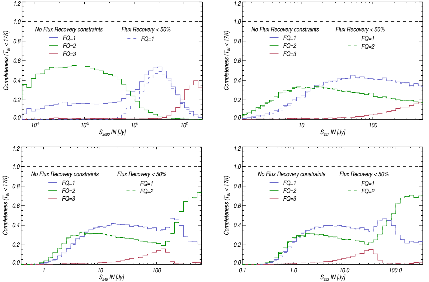
Fig. 5. Completeness (computed on a restricted sample of sources with injected temperature below 17 K) as a function of the injected flux density in the IRAS 3 THz (top left panel) and Planck upper frequency bands, 857 GHz (top right panel), 545 GHz (bottom left panel), and 353 GHz (bottom right panel). It is shown per-category of flux density quality, i.e., FQ = 1, 2 and 3 categories (blue, green and pink, respectively). The completeness is also computed on a more restricted sample of sources with injected temperature below 17 K and with a flux density accuracy better than 50% (dashed lines).
