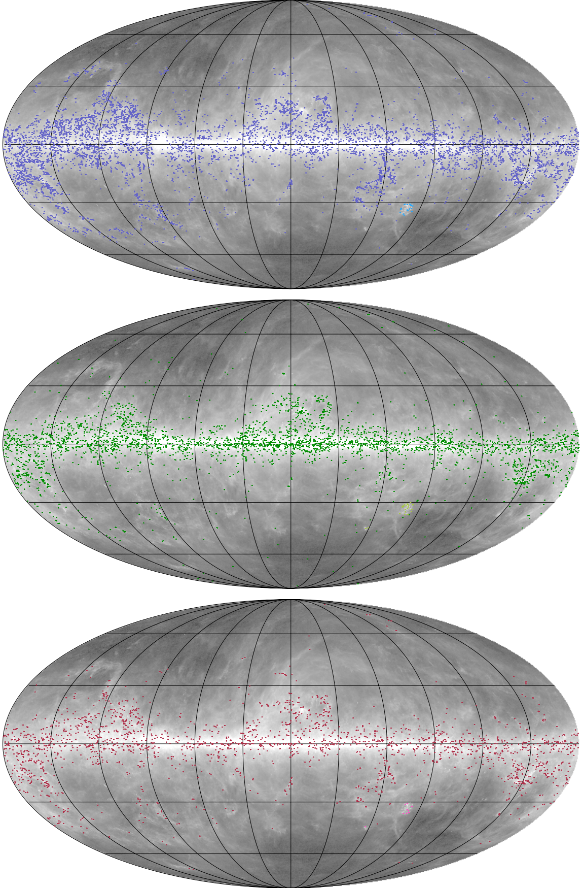
Fig. 2. All-sky distribution of the PGCC sources according to their FLUX_QUALITY category: “Reliable flux densities” (FQ = 1, top panel ), “Missing 3 THz flux density” (FQ = 2, middle panel ) and “Detection only” (FQ = 3, bottom panel ). Sources located in the LMC and SMC are also shown in light colours.
