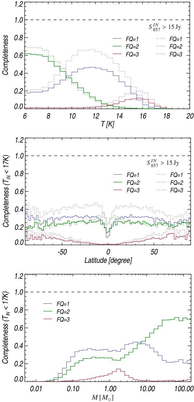
Fig. 4. Completeness as a function of the input temperature ( top panel ), latitude ( middle panel ), and mass ( bottom panel ) of the injected sources. For the latitude and mass cases, the input temperature was lower than 17 K. In addition, when considering the dependence of completeness on mass, all the sources are assumed to be at 100 pc from the Sun. Each panel shows the distributions obtained from selecting only the sources in a given FLUX_QUALITY category. In particular, FQ = 1, 2 and 3 correspond to the blue, green and pink curves, respectively. Finally, the dotted line in each panel denotes the completeness for the sample of sources with input flux density S_{857}^{IN} > 15 Jy.
