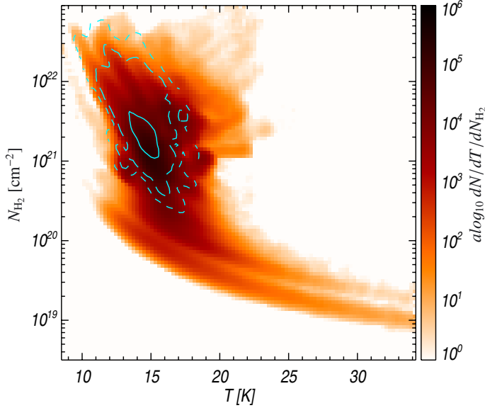
Fig. 15. Temperature vs. column density two-dimensional distribution for all PGCC cold clumps followed up by Herschel in the HKP-GCC programme. The plotted data points are identified as IN and OUT: IN points are located inside the Planck clump solid angle, while the OUT points are located outside. The distribution of the OUT points is shown in colour, while the distribution of the IN points is denoted by cyan contours at three different levels: 10, 50 and 90% of the maximum.
