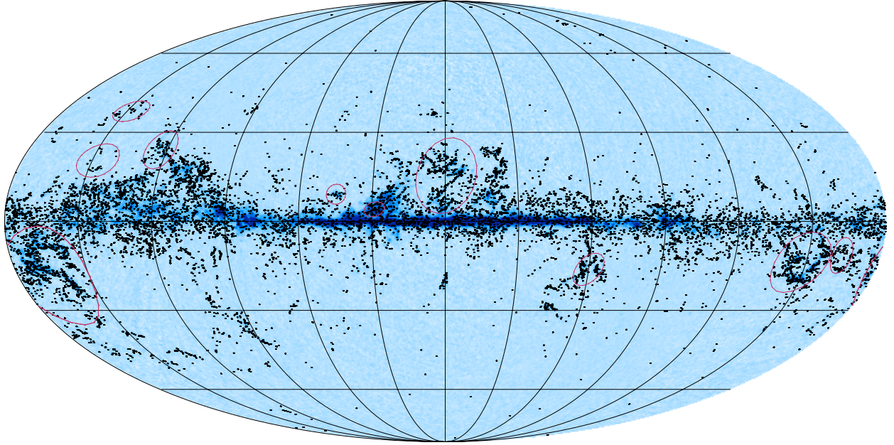
Fig. B.1. All-sky distribution of the PGCC sources with FQ=1 or 2 , displayed over the Planck ^{12}\text{CO } J = 1 \rightarrow 0 map ranging from -5 to 30 \text{ K km s}^{-1} . The locations of the molecular complexes used in the distance estimate procedure are shown as red circles.
