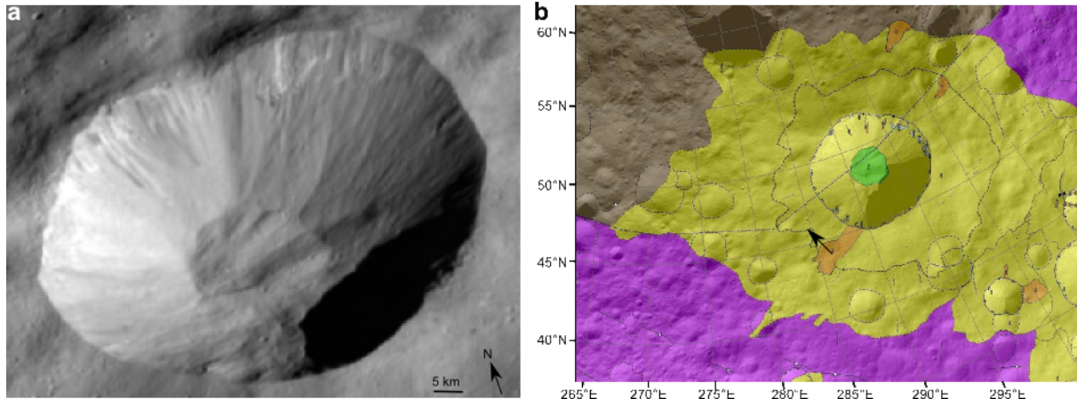
Fig. 5: Mamilia crater. a – Non-projected image from Dawn FC. b – Geological map (Ruesch et al., 2014a). Materials with different albedos compose the upper part of northern wall, while mass-wasted materials lie on the floor.
