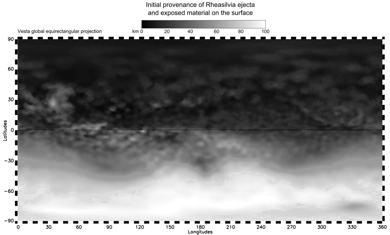
Fig. 3: Global map of Rheasilvia ejecta depth model, 0-100 km (Jutzi et al., 2013). This equirectangular projection is in the Claudia system of coordinates that is the standard for maps of Vesta generated by the Dawn team, and therefore is shifted by 150E to the East with respect to the IAU system (International Astronomical Union). Note also that projections of the maps by Jutzi et al. (2013) were not internally consistent in the publication. In our version, the deepest ejecta correspond to Rheasilvia and Veneneia basins, using the Digital Elevation Model (DEM) derived from Dawn data.
