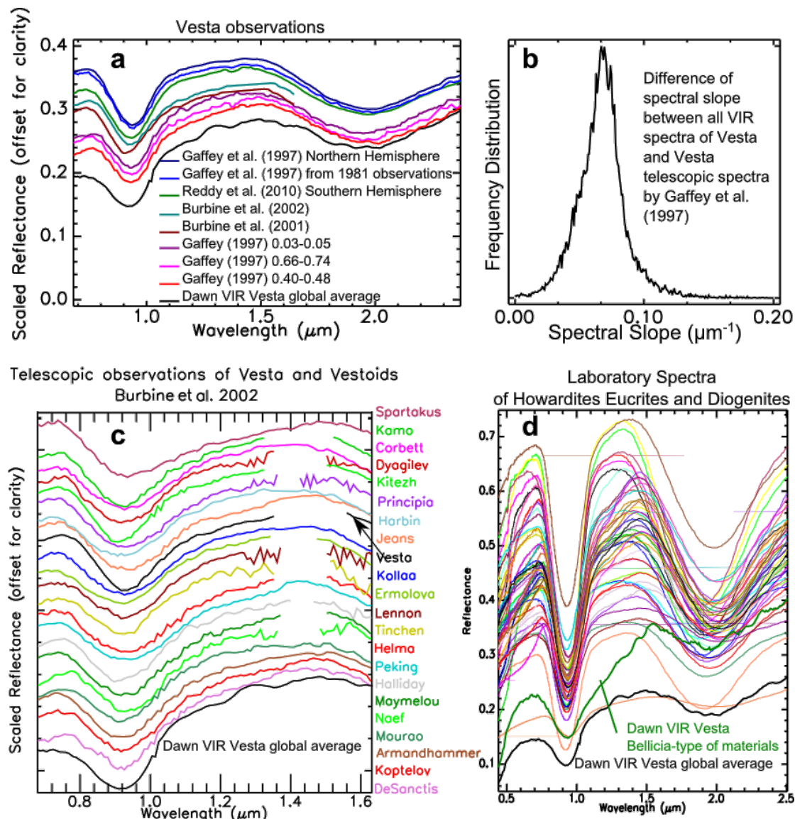
Fig. 7: Evidence of a more positive spectral slope in Dawn VIR observations of Vesta than in any other spectral dataset of Vesta, Vestoids or HED samples. a – Spectra of Vesta’s surface. b – Histogram showing that VIR spectra have a more positive slope than the telescopic spectrum acquired by Gaffey et al. (1997) in 1981, which has the most positive slope among all telescopic spectra. c – Telescopic spectra of Vestoids compared to Dawn VIR at Vesta. d – Laboratory spectra of HED samples compared to Dawn VIR at Vesta.
