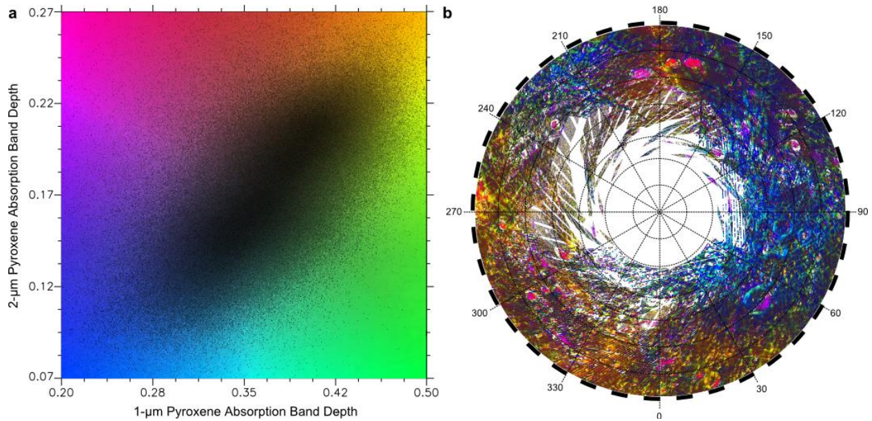
Fig. 14: Variations of the two pyroxene absorption band depth for the northern regions of Vesta. a – Two-dimensional scatter plot of VIR data. The color scale in the background of the data cloud is the key plot for the map on the right. b – North polar view of the two pyroxene absorption band depths, using the color key represented on the left.
