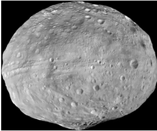
Fig. 1: Vesta as observed by the Dawn FC on September 22, 2011, pointing at the equator, showing the different shapes of the two hemispheres. While the northern hemisphere is close to an ellipsoid, the southern hemisphere is largely shaped by the Rheasilvia basin and its central peak, an impact feature that is not hydrostatically compensated.
