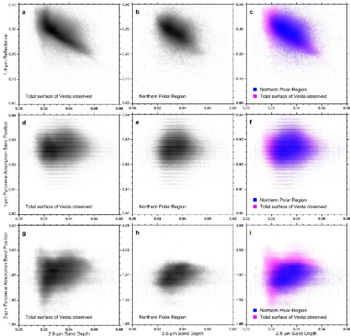
Fig. 10: 2-D scatter plots of various spectral properties of the surface of Vesta as function of the 2.8-μm band depth. First row (a, b, c): 1.4-μm reflectance. Second row (d, e, f): Pyroxene 1-μm absorption band position.
