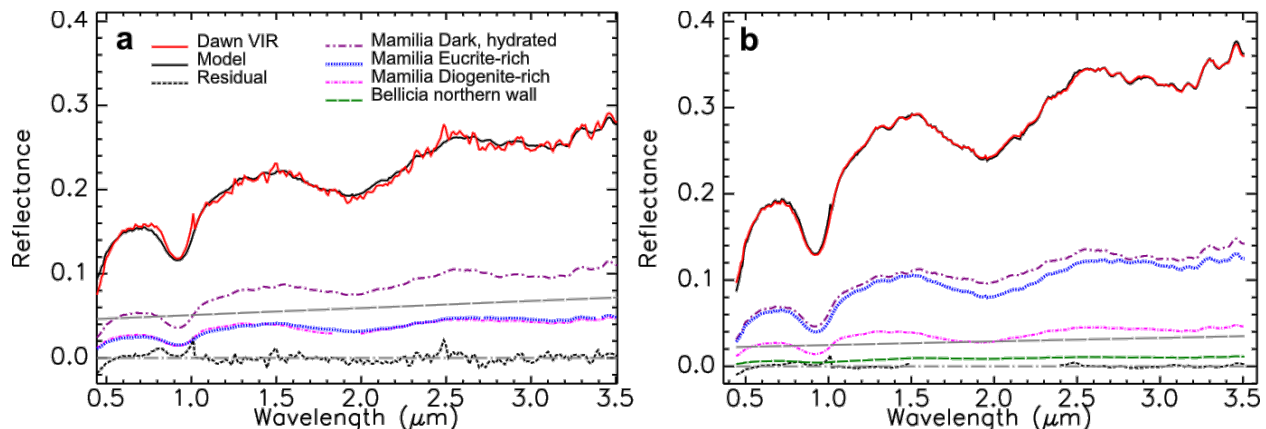
Fig. 9: Example of spectral fitting using MELSUM. All endmember spectra shown are weighted by their respective mixing coefficient, which explains the differences between the two panels of the figure. The sum of all spectral endmembers as represented equals the modeled spectrum (black solid curve). a – Dark materials from a region between Caesaria and Arruntia craters. b – Average spectrum of Vesta.
