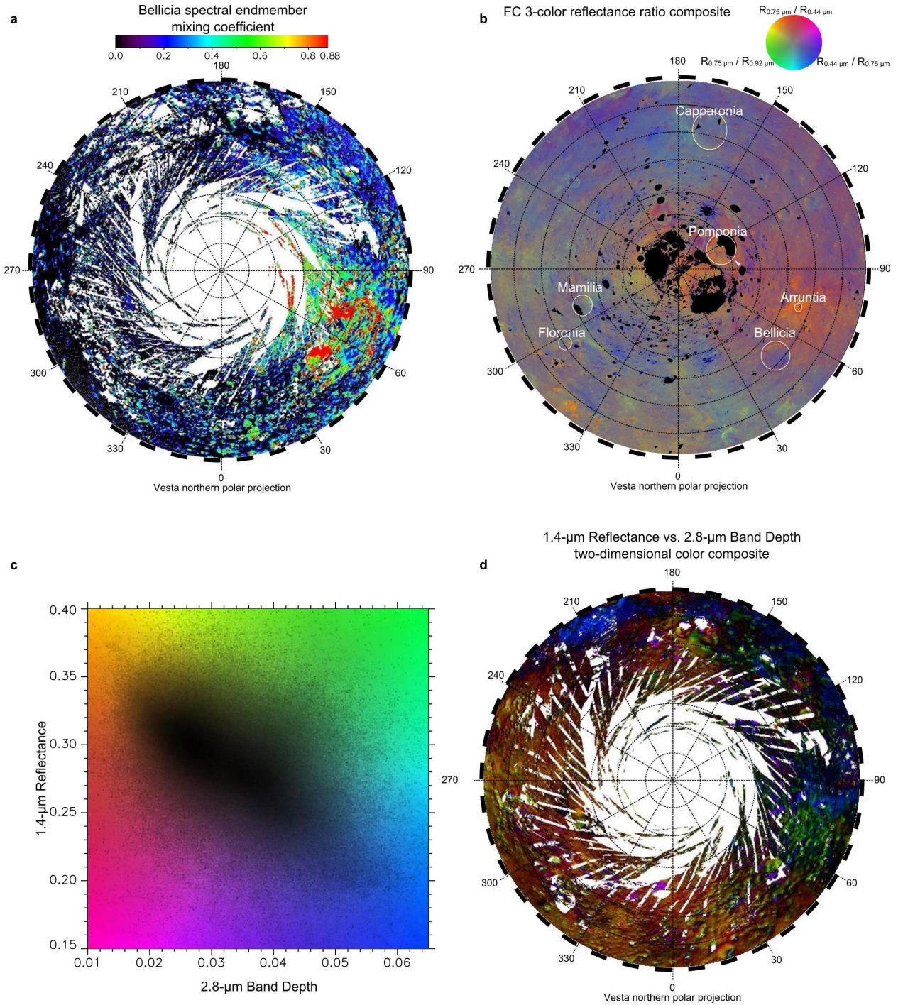
Fig. 16: North polar view of Vesta surface composition. a – Mixing coefficient distribution of the Bellicia-type of material calculated with MELSUM. b – Three color composite from FC reflectance ratios. Red: R_{0.75 \mu\text{m}} / R_{0.44 \mu\text{m}} . Green: R_{0.75 \mu\text{m}} / R_{0.92 \mu\text{m}} . Blue: R_{0.44 \mu\text{m}} / R_{0.75 \mu\text{m}} . c – Two-dimensional scatter plot of 1.4 \mu\text{m} reflectance vs. 2.8 \mu\text{m} band depth. The color scale in the background and the level of shade are the key plot for the map (d) on the lower right. d – Color composite of 1.4 \mu\text{m} reflectance vs. 2.8 \mu\text{m} band depth, as defined by the color scale on the lower left (c). Regions in green pixels indicate areas with relatively high albedo and deep 2.8 \mu\text{m} band. They define a spatially coherent region including the Bellicia, Arruntia and Pomponia craters.
