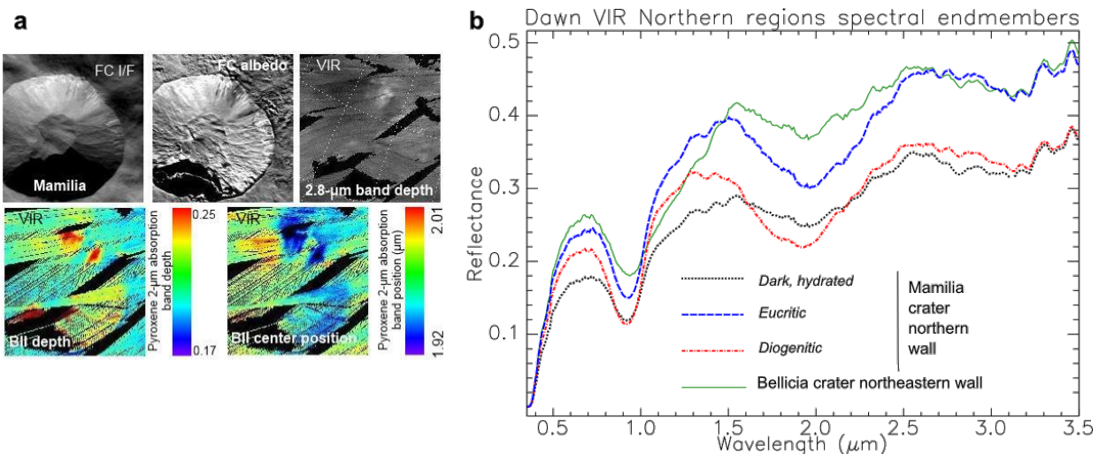
Fig. 8: Selection process of spectral endmembers from Mamalia crater northern wall. a – Identification of areas with extreme compositions from maps of spectral parameters. b – VIR spectral endmember collection from Mamalia crater (diagenitic, eucritic and dark hydrated materials) and Bellicia wall (olivine-like component).
