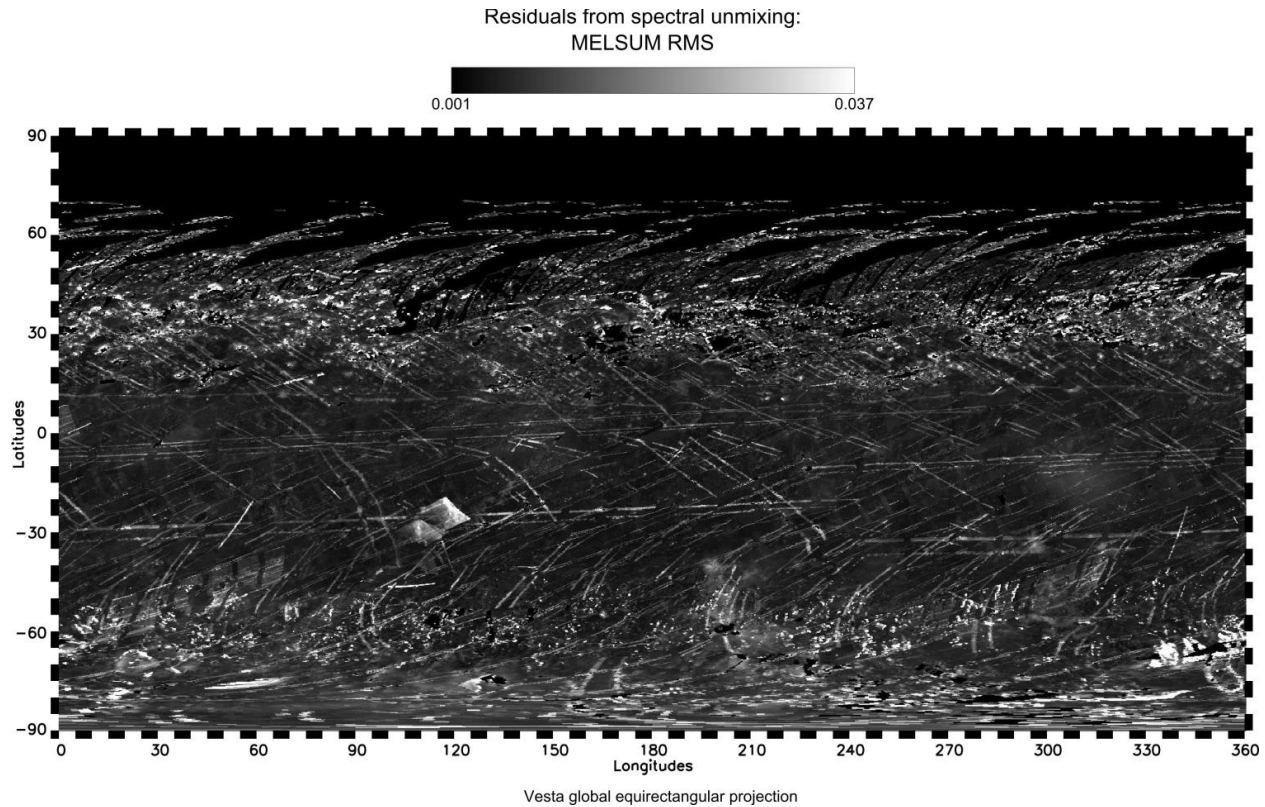
Fig. 15: Global map of Vesta in equirectangular projection of residuals (RMS) from MELSUM performed on VIR entire dataset, using spectral endmembers from Mamilia crater northern wall (diogenitic, eucritic and dark hydrated materials) and Bellicia wall (olivine-like component).
