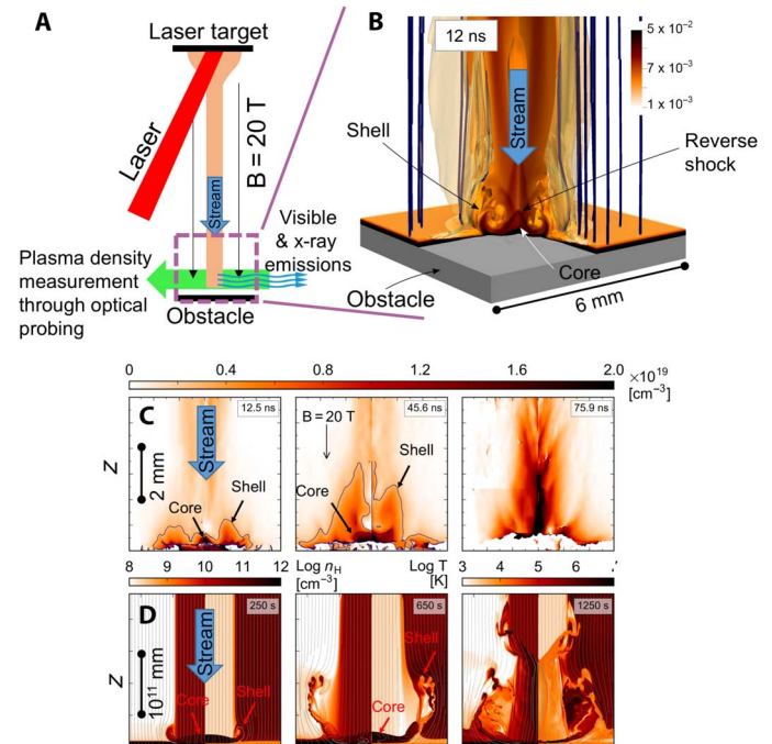
Fig. 1. Laboratory investigation of magnetized accretion dynamics and comparison with scaled astrophysical simulation of the same phenomenon highlighting the formation of a shocked core and of a surrounding shell. (A) Arrangement of the laboratory experiment and of the diagnostics. (B) Snapshot of the modeling of the laboratory experiment by the GORGON code (shown is the mass density in kg/m 3 ). (C) Measured maps, at different times (as indicated), of laboratory plasma electron density, embedded in a homogeneous and steady 20-T magnetic field. The contours displayed on the first two panels highlight the core (contour at 10^{19} cm -3 ) and the shell (contour at 3 \times 10^{18} cm -3 ). Here, the obstacle is a CF 2 target, whereas the stream is generated from a laser-irradiated PVC (C 2 H 3 Cl) n target. (D) Simulated plasma density (left-half panels) and temperature (right-half panels) maps, also at different times, and extracted from a 2D astrophysical simulation (using the PLUTO code). In all panels, the initial magnetic field is uniform and oriented along the z axis; the white (resp. black) lines in (A) and (C) (resp. B) represent the magnetic field lines. In all, the obstacle/chromosphere is located at the bottom, at z = 0 , and t = 0 corresponds to the moment when the stream hits the obstacle/chromosphere.
