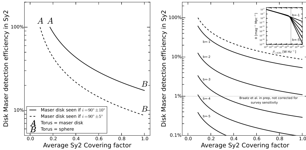
Figure 1. Left. Disk maser detection efficiency as a function of average Sy2 covering factor, assuming two different thickness for the maser disk. Right. Effect of different slopes b of the 1.4 GHz LF (inset) on the intrinsic detection efficiency.
