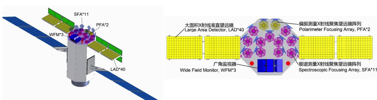
Figure 1. The baseline design of the mission is schematically summarized here. The left panel shows an artistic view of the eXTP satellite, with the payload module tower and four LAD panels. In the right panel the top view of the scientific payload is shown. The current configuration of the mission includes 11 telescopes of the SFA, 2 telescopes of the PFA, 40 modules for the LAD and 3 WFM units, each composed of 2 cameras.
