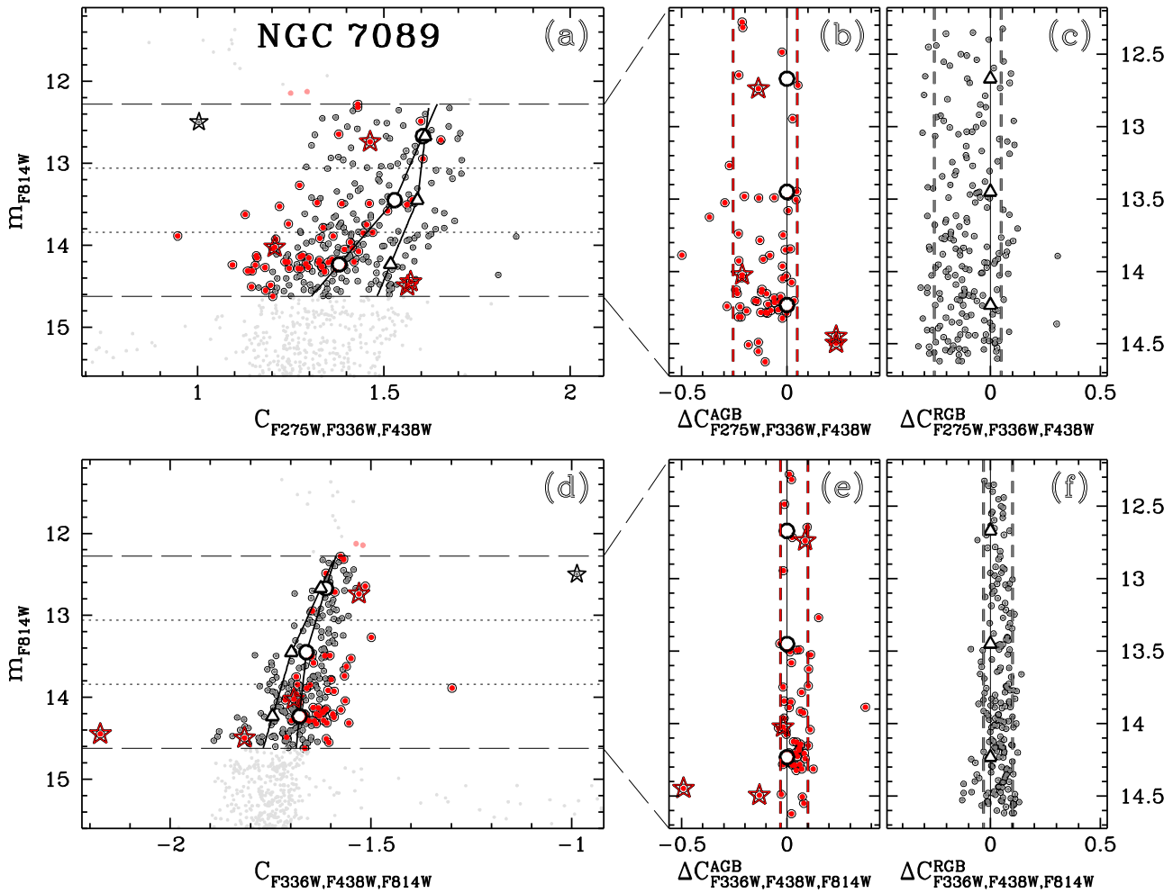
Figure 12. Determination of the width of AGB and RGB stars of NGC 7089. Panel (a): m_{F814W} vs. C_{F275W,F336W,F438W} CMD of the cluster AGB (red points) and RGB/HB (gray points) stars included in the selected F814W magnitude interval, marked by long-dashed horizontal lines. AGB stars brighter than the selected luminosity threshold are represented as light-red points. Anomalous AGB candidates have been marked with a red star symbol, while the only post-EAGB candidate star has been marked with a black star symbol. Panels (b), (c): verticalized CMDs of the cluster AGB (panel (b)) and RGB (panel (c)) stars, where the horizontal displacement between the two dashed vertical lines represents the corresponding observed width. Panels (d)–(f): same as panels (a)–(c) but for the pseudo-color C_{F336W,F438W,F814W} .
