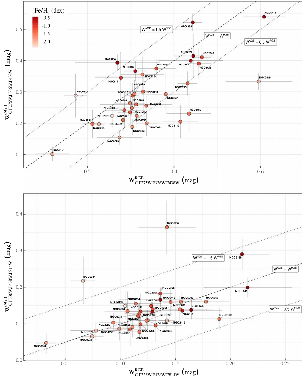
Figure 14. Top: W_{C F275W,F336W,F438W}^{AGB} vs. W_{C F275W,F336W,F438W}^{RGB} of the 35 GCs in Table 1. The color of each point maps the cluster’s metallicity, according to the scale reported in the legend. Bottom: W_{C F336W,F438W,F814W}^{AGB} vs. W_{C F336W,F438W,F814W}^{RGB} of the same clusters. The reference dashed and dotted lines overlotted in each panel represent the relations indicated by the corresponding labels.
