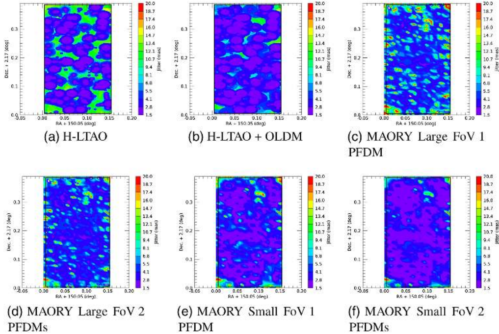
Fig. 9 Jitter with H-LTAO (on axis) or with MAORY (averaged on the scientific FoV) for the COSMOS field. The jitter is limited to 20 mas for a better display. The black lines indicate the area used for the SC computation.
