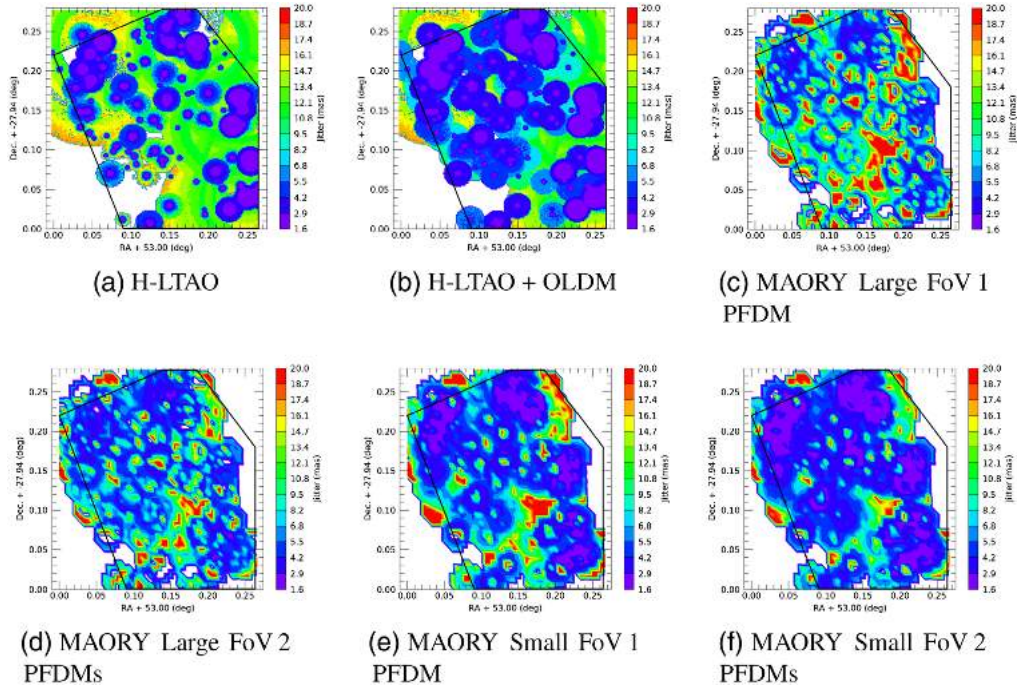
Fig. 15 Jitter with H-LTAO (on axis) or with MAORY (averaged on the scientific FoV) for the GOODS-S field. The jitter is limited to 20 mas for a better display. The black lines indicate the area used for the SC computation.
