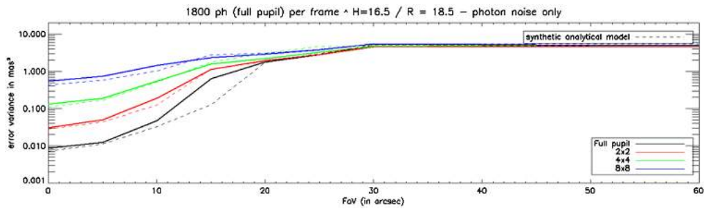
Fig. 26 Evolution of the noise variance (in \text{mas}^2 ) as a function of the FoV position. Solid line = simulation, dotted line = analytical expression in the good SR regime, dashed-line = FWHM regime.
