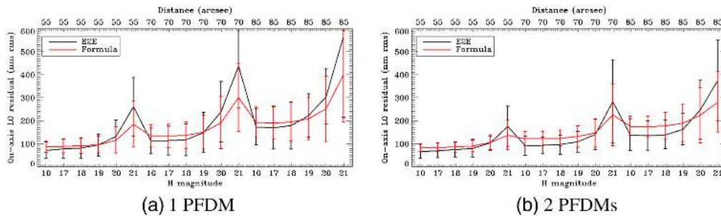
Fig. 24 Comparison of the LO residual on axis from the E2E simulations and from the formula. (a) With one PFDM and (b) with two PFDMs. All asterisms are equilateral triangles, with all the stars at the same distance and the same magnitude (indicated on the x axis).
