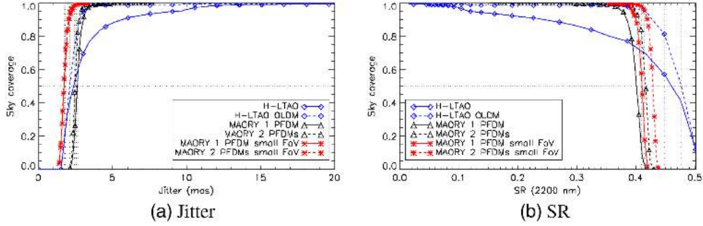
Fig. 6 SC with H-LTAO or with MAORY at l = 90 deg, b = -30 deg. The jitter/SR is on axis for H-LTAO and averaged on a 1 arcmin diameter FoV (large FoV) or on a 20'' diameter FoV (small FoV) for MAORY.
