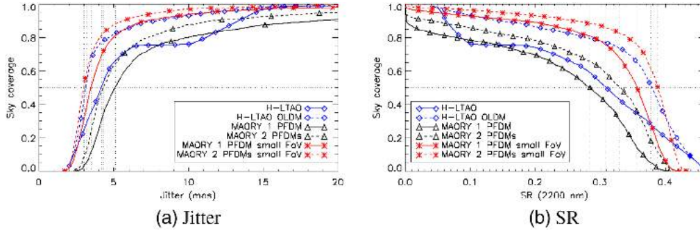
Fig. 21 SC with H-LTAO or with MAORY for the UDS field. The jitter/SR is on axis for H-LTAO and averaged on a 1 arcmin diameter FoV (large FoV) or on a 20" diameter FoV (small FoV) for MAORY.
