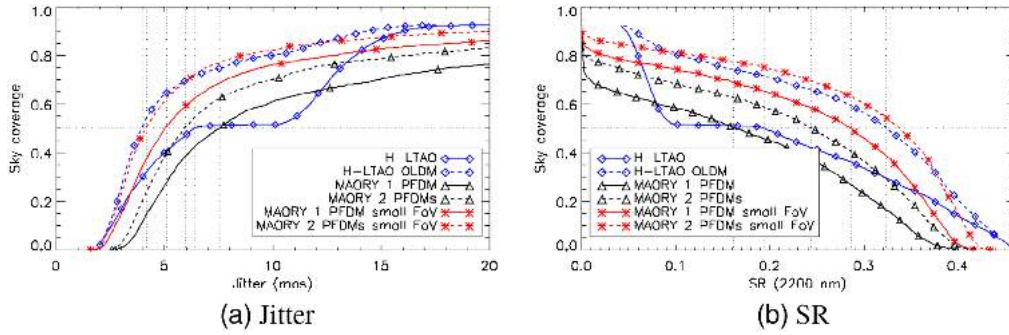
Fig. 22 SC with H-LTAO or with MAORY for the GOODS-S field. The jitter/SR is on axis for H-LTAO and averaged on a 1 arcmin diameter FoV (large FoV) or on a 20" diameter FoV (small FoV) for MAORY.
