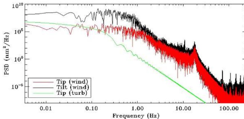
Fig. 1 Temporal PSDs of the TT due to the windshake on M2, compared with the turbulence PSD. The PSDs are computed from the time series using a Hanning window.
