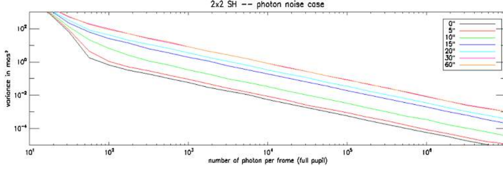
Fig. 4 Example of noise computed for a 2 \times 2 SHWFS, for different level of fluxes, and different position of the NGS in the field, in the case of an LTAO correction without OLDLM.
