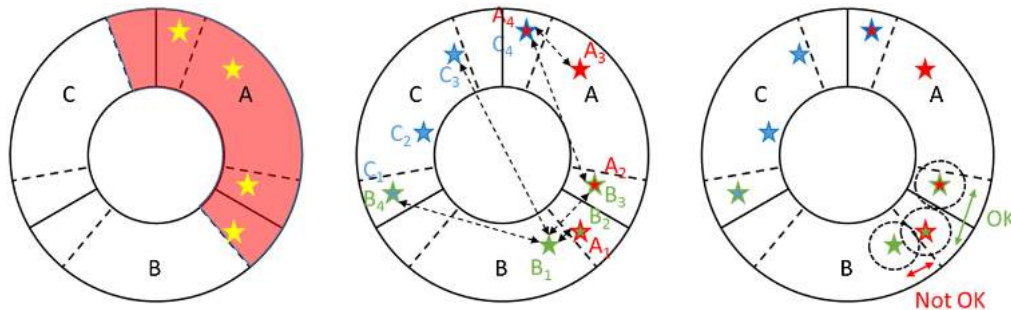
Fig. 2 Method to detect a valid configuration in the case of MAORY. The sensors' dedicated working areas are delimited by the solid lines, while the dashed lines indicate the possible extension of these areas. Between two dashed lines, we thus have an overlap zone between two sensors. Steps are, from left to right: (1) register all the stars under the limiting magnitude reachable by each sensor (remove those too close to the center to avoid vignetting). In this figure, we show the example for WFS A (the same is done for WFSs B and C). The red color shows the total area eventually reachable by the WFS A. Here, the star symbols are the potential NGSs for this sensor. (2) Compute distances between the registered stars. Here, the stars are color-coded as a function of which sensor can reach it (filling color = dedicated zone, contour color = overlap zone): red for WFS A, green for WFS B, and blue for WFS C. They are also named accordingly as indicated in the figure (a star reachable by two sensors will have two names). (3) Check the combinations that avoid collisions of the pick-off mirrors. For example, B2/A1 cannot be selected together with B1, but it can be selected together with B3.
