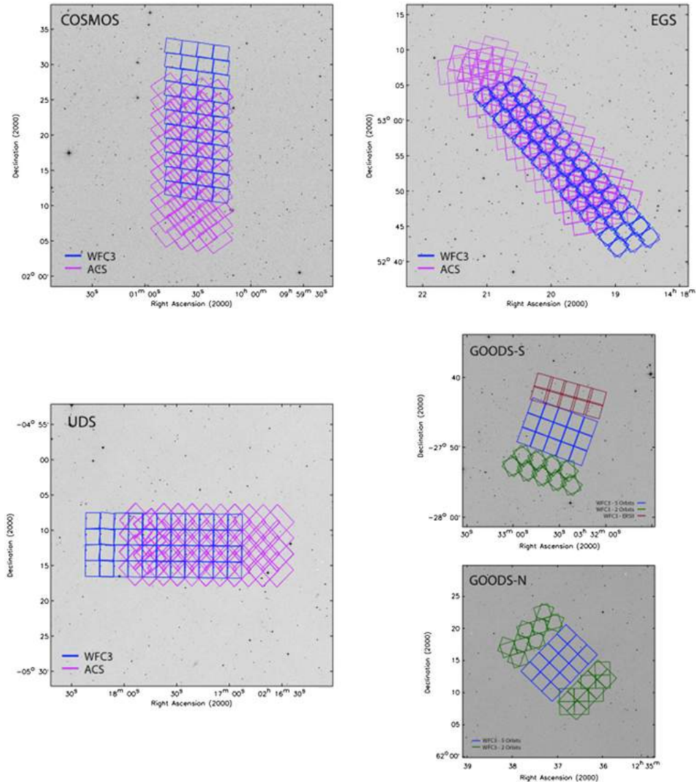
Fig. 8 Cosmological fields considered in this section. Taken from Ref. 20.
