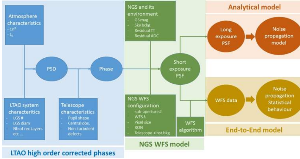
Fig. 3 Global scheme of the E2E TT noise estimation.
