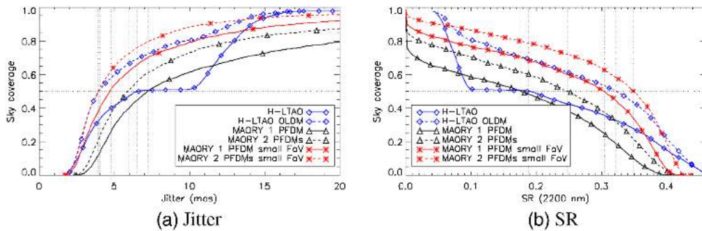
Fig. 20 SC with H-LTAO or with MAORY for the EGS field. The jitter/SR is on axis for H-LTAO and averaged on a 1 arcmin diameter FoV (large FoV) or on a 20" diameter FoV (small FoV) for MAORY.
