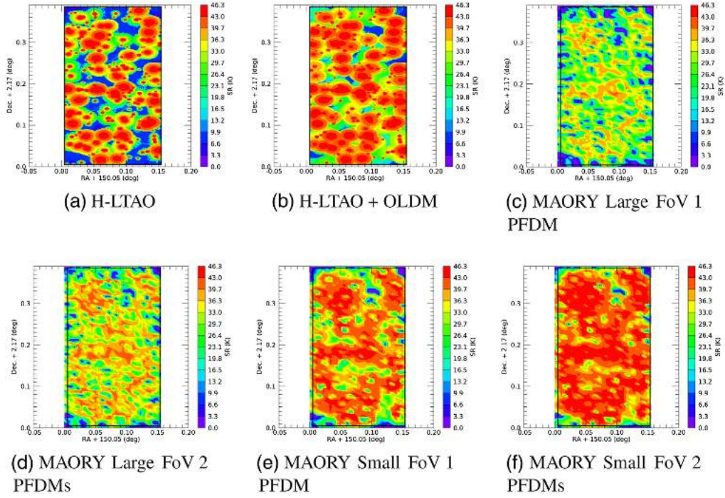
Fig. 10 SR in K band with H-LTAO (on axis) or with MAORY (averaged on the scientific FoV) for the COSMOS field. The black lines indicate the area used for the SC computation.
