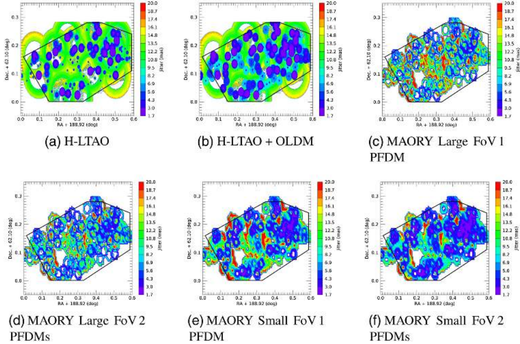
Fig. 17 Jitter with H-LTAO (on axis) or with MAORY (averaged on the scientific FoV) for the GOODS-N field. The jitter is limited to 20 mas for a better display. The black lines indicate the area used for the SC computation.
