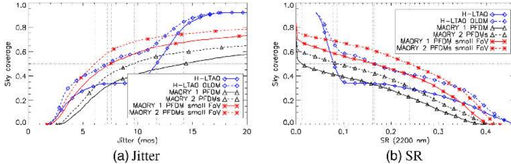
Fig. 23 SC with H-LTAO or with MAORY for the GOODS-N field. The jitter/SR is on axis for H-LTAO and averaged on a 1 arcmin diameter FoV (large FoV) or on a 20" diameter FoV (small FoV) for MAORY.
