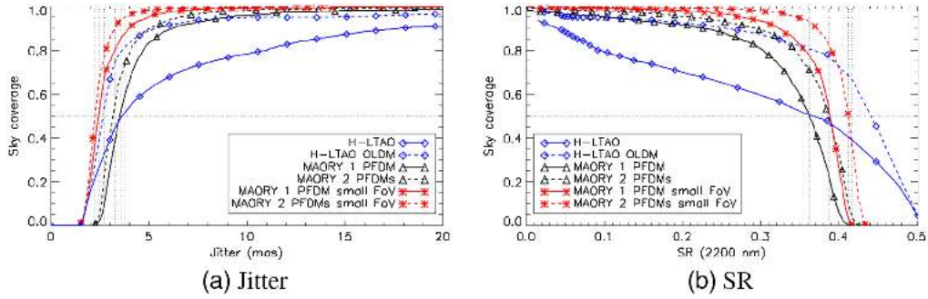
Fig. 7 SC with H-LTAO or with MAORY at l = 90 deg, b = -60 deg. The jitter/SR is on axis for H-LTAO and averaged on a 1 arcmin diameter FoV (large FoV) or on a 20'' diameter FoV (small FoV) for MAORY.
