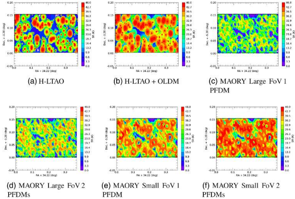
Fig. 14 SR in K band with H-LTAO (on axis) or with MAORY (averaged on the scientific FoV) for the UDS field. The black lines indicate the area used for the SC computation.
