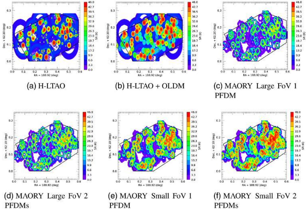
Fig. 18 SR in K band with H-LTAO (on axis) or with MAORY (averaged on the scientific FoV) for the GOODS-N field. The black lines indicate the area used for the SC computation.
