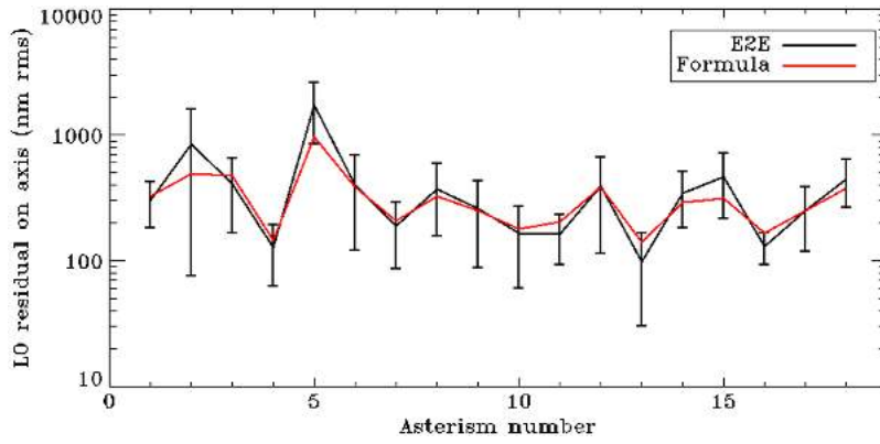
Fig. 25 Comparison of the LO residual on axis from the E2E simulations and from the formula, for 18 random asterisms and two DMs.
