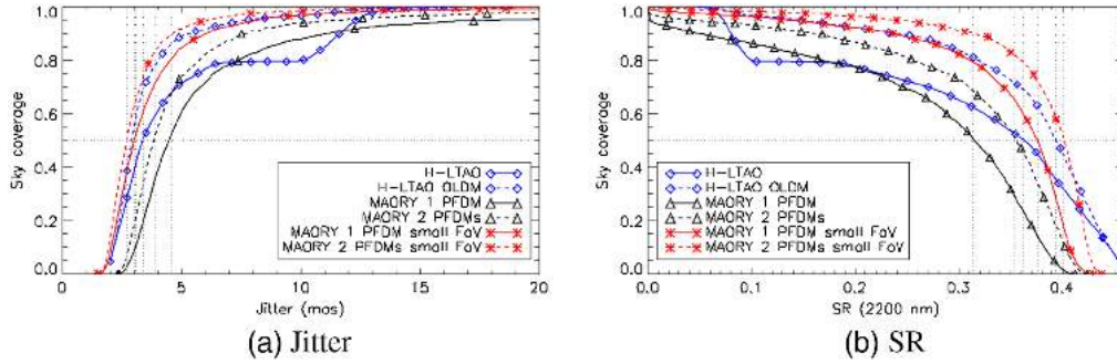
Fig. 19 SC with H-LTAO or with MAORY for the COSMOS field. The jitter/SR is on axis for H-LTAO and averaged on a 1 arcmin diameter FoV (large FoV) or on a 20" diameter FoV (small FoV) for MAORY.
