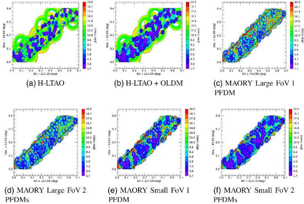
Fig. 11 Jitter with H-LTAO (on axis) or with MAORY (averaged on the scientific FoV) for the EGS field. The jitter is limited to 20 mas for a better display. The black lines indicate the area used for the SC computation.
