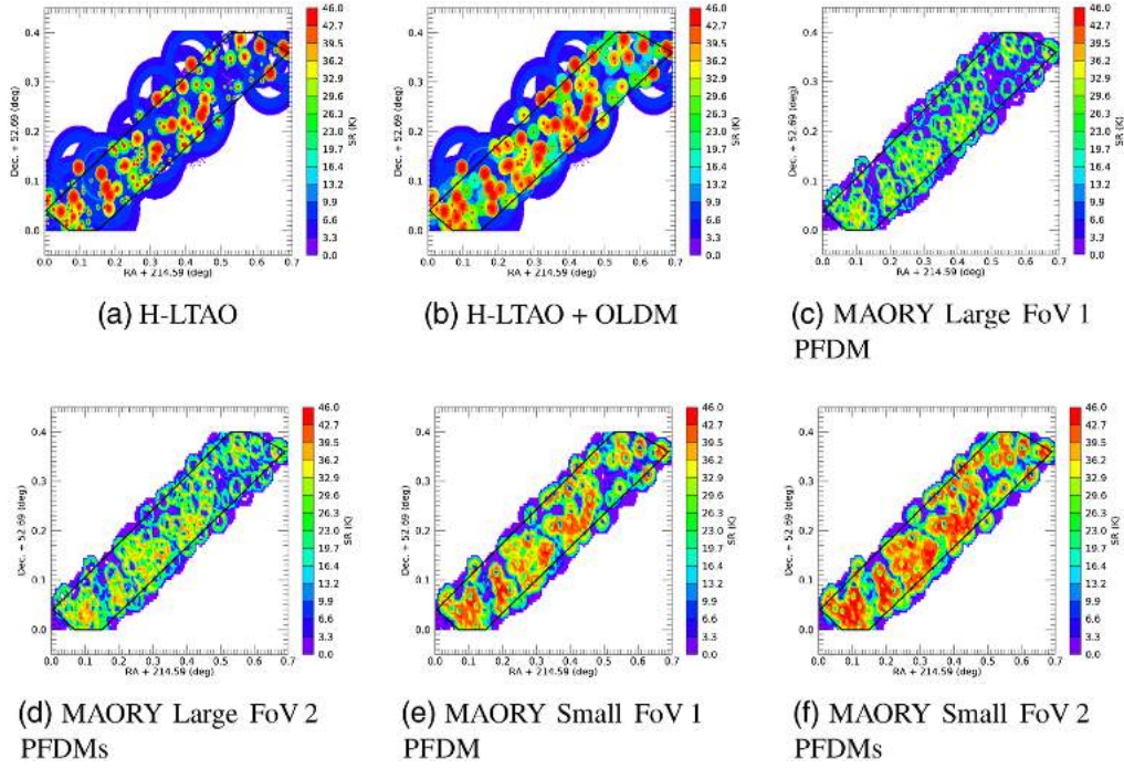
Fig. 12 SR in K band with H-LTAO (on axis) or with MAORY (averaged on the scientific FoV) for the EGS field. The black lines indicate the area used for the SC computation.
