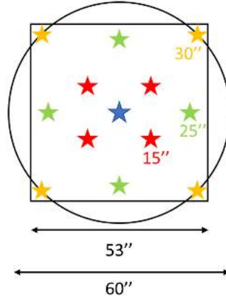
Fig. 5 Directions used for the jitter/SR computation in the FoV of 60'' diameter. The square of side 53'' corresponds to the large MICADO FoV. The stars are distributed as follows: one star on axis, four stars at 15'', four stars at 25'', and four stars at 30''. When the small MICADO FoV is considered (20×20''), we average from one star on axis and four stars at 10'' (placed in the same manner as the four stars at 15'').
