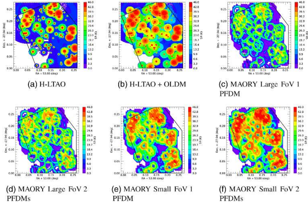
Fig. 16 SR in K band with H-LTAO (on axis) or with MAORY (averaged on the scientific FoV) for the GOODS-S field. The black lines indicate the area used for the SC computation.
