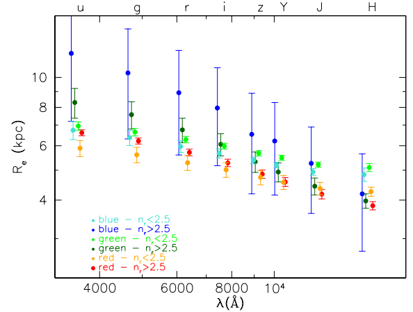
Figure 13. Median effective radius as a function of wavelength for galaxies of different colour and Sérsic index. Red, dark green and blue symbols represent high- n galaxies; orange, light green and turquoise symbols low- n galaxies. Error bars represent the uncertainty on the median. The median effective radius depends on wavelength. Small offsets in wavelength have been applied to all points for clarity. Low- n samples display similar behaviour, while the high- n samples show stronger, and more varied, trends.
