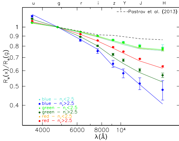
Figure 16. Median values of \mathcal{R}_g^x as a function of wavelength \lambda , where x denotes the band corresponding to wavelength \lambda . As indicated by the legend, red, dark green and blue symbols and lines represent high-n galaxies; orange, light green and turquoise symbols and lines represent low-n galaxies. Median \mathcal{R}_g^x = R_e(x)/R_e(g) are plotted by points. Error bars give the uncertainty on the median. Lines plot median[ R_e(x) ]/median[ R_e(g) ], i.e. the points from Fig. 13 normalized to the g band. Small offsets in wavelength have been applied to all points for clarity. The black dashed line represent the wavelength dependence of \mathcal{R} for a disc population due to the effects of dust, as predicted by Pastrav et al. (2013a). We do not plot the prediction for the u band since it has not been calculated in the model, but it is a linear interpolation from the B band to the near-UV. The trends for the low-n samples are indistinguishable, irrespective of galaxy colour. The high-n samples show steeper trends which depend on colour.
