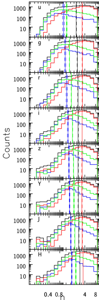
Figure 4. Sérsic index distribution for our full sample (black line) and for galaxies in each of our colour subsamples ( red, green, blue ). Each panel shows the distribution in a different band: ugrizYJH . The median of each distribution, and its uncertainty, are indicated by vertical solid and dashed lines, respectively. The median Sérsic index for red galaxies does not depend on wavelength, while for our green and blue subsamples, the Sérsic index increases significantly towards redder wavelengths.
