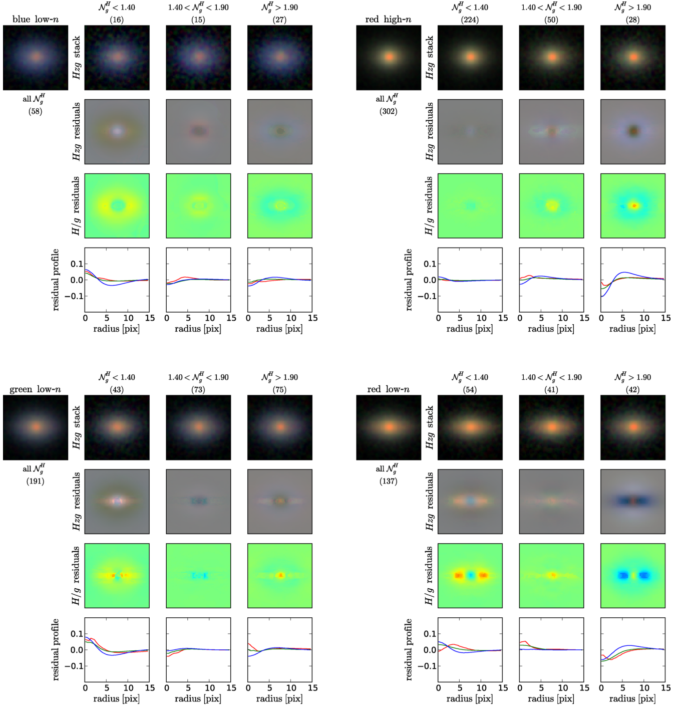
Figure 20. Stacked \mathcal{N}_g^H gradients, for galaxies with similar colour and Sérsic index. For each set of stacks, we divide the galaxy sample into three groups, by cutting at \mathcal{N}_g^H = 1.4 and 1.9 (see text for details). In each subplot, the top panels show the stacked images using the Hzg bands, the second-to-top panels show the residuals, the second-to-bottom panels show the ratio of the H and g residuals and the bottom panels show the radial profiles of the H , z and g residuals. Numbers in parenthesis are the numbers of galaxies used in each stack. The Hzg stack and residuals are displayed using the colour-preserving method of Lupton et al. (2004). The stack images have an asinh stretch, while the residual images are shown with a linear stretch. The H/g residuals image has a false-colour scale, where green corresponds to equal residuals in H and g , red indicates that the H residuals are brighter than those in g and blue indicates the converse. Each image is 30 pixels across. The radial profiles show the fractional difference in flux between this image stack and that of all objects in the same colour and Sérsic index subsample. It is clear that galaxies with higher \mathcal{N} are fainter and redder in the centre, but bluer at intermediate radii, and vice versa for lower values of \mathcal{N} . We do not show images for blue and green high- n galaxies because they are too few to produce meaningful stacked images.
