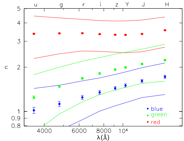
Figure 5. Median Sérsic index as a function of wavelength for our red, green and blue galaxy subsamples. Error bars represent the uncertainty on the median. Solid lines indicate the 16th- and 84th-percentiles of the distribution. The red subsample clearly behaves differently to our green and blue subsamples: the Sérsic index of red galaxies is very stable across all optical–NIR wavelengths, while Sérsic index shows a steady increase with wavelength for bluer galaxies.
