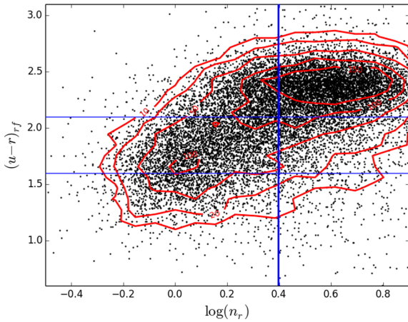
Figure 3. (u-r)_f versus n_r for the galaxies in our sample. Lines illustrate the cuts we apply to divide the galaxies by colour and Sérsic index.
