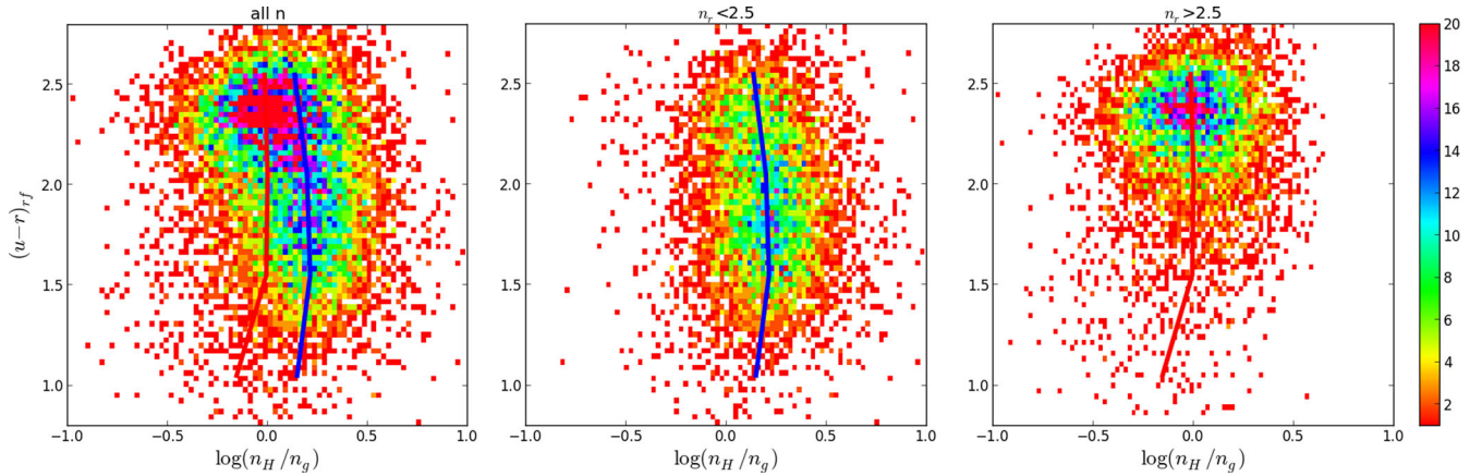
Figure 7. Density map of (u-r) colour versus the ratio of the H -band Sérsic index and g -band Sérsic index, defined here as \mathcal{N}_g^H = n_H/n_g . The left-hand panel displays all galaxies together, while centre and right panels show only galaxies with low and high Sérsic indices, respectively. The median \mathcal{N}_g^H as a function of colour is also plotted, for both the low-n (blue line) and high-n (red line) samples. These two populations show different distributions, indicating that their constituent galaxies possess different internal structures. High-n galaxies have \mathcal{N} \sim 1 , indicating that the central concentration of their profile tends not to change with wavelength. On the other hand, low-n galaxies generally display peakier profiles in the red, particularly those with intermediate colour.
