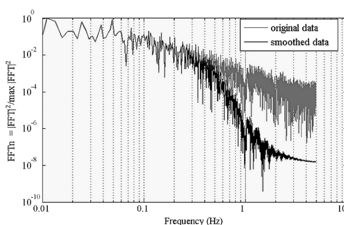
Fig. 6. Normalized power of two FFT norms ( FFT_n ) of the discharge signal Q(t) , for a velocity ratio V_t/U = 1.8
