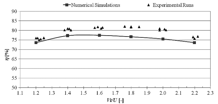
Fig. 7. Plot of the efficiency versus the velocity ratio V_t/U ; comparison between the experimental and numerical results
