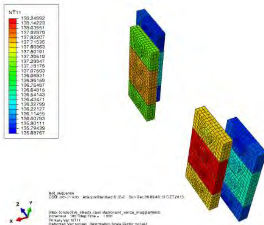
Figure 13-44 Main MLI Shield internal and external temperature distribution [K]
