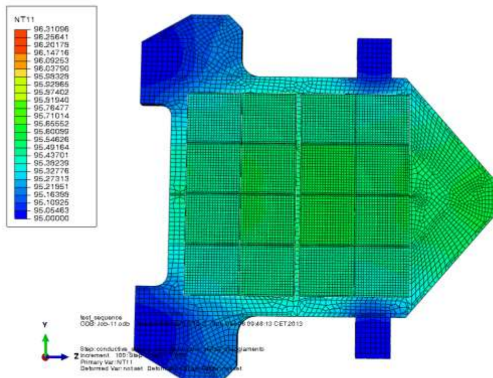
Figure 13-30 Detectors and CSS front temperature distribution [K]
