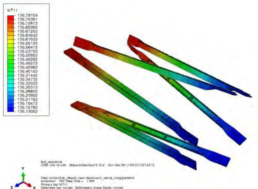
Figure 13-98 Structural beams temperature distribution [K]
