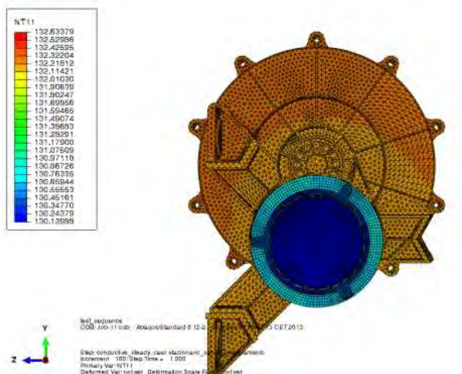
Figure 13-1 P1 and CaLA assembly temperature distribution [K]
