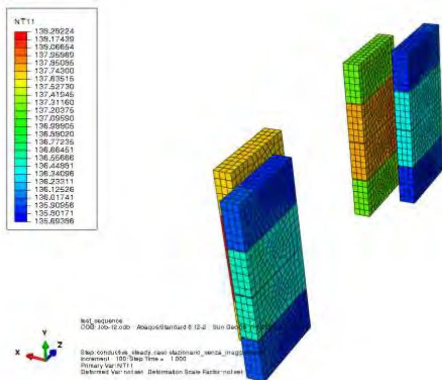
Figure 13-96 Sidcars temperature distribution [K]
