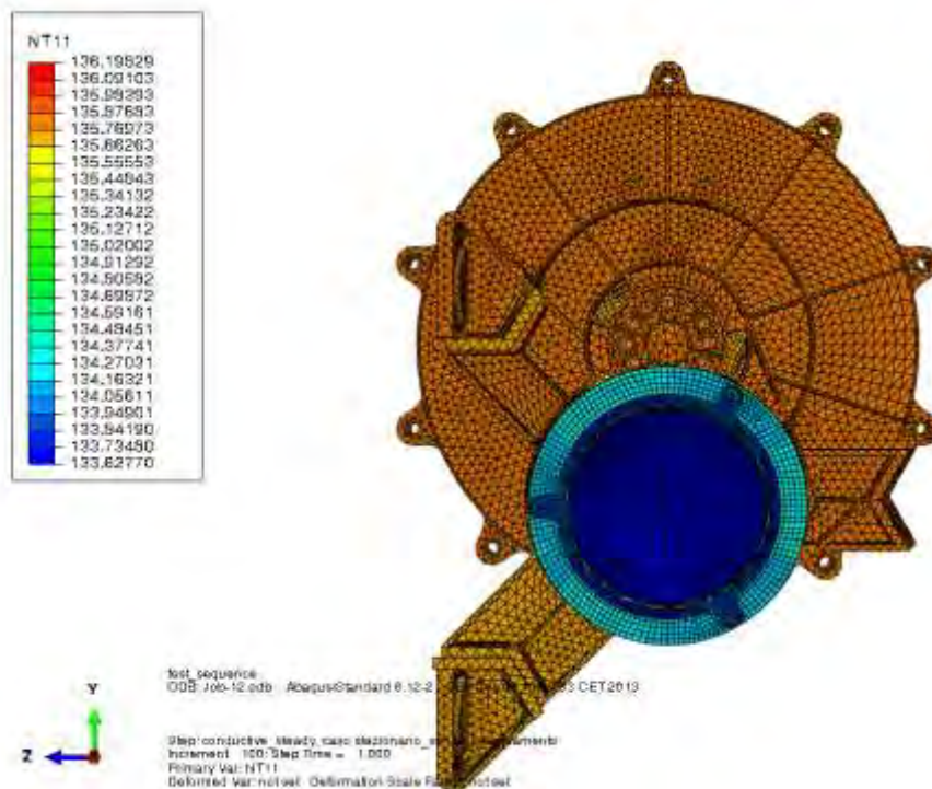
Figure 13-50 P1 and CaLA assembly Temperature distribution [K]
