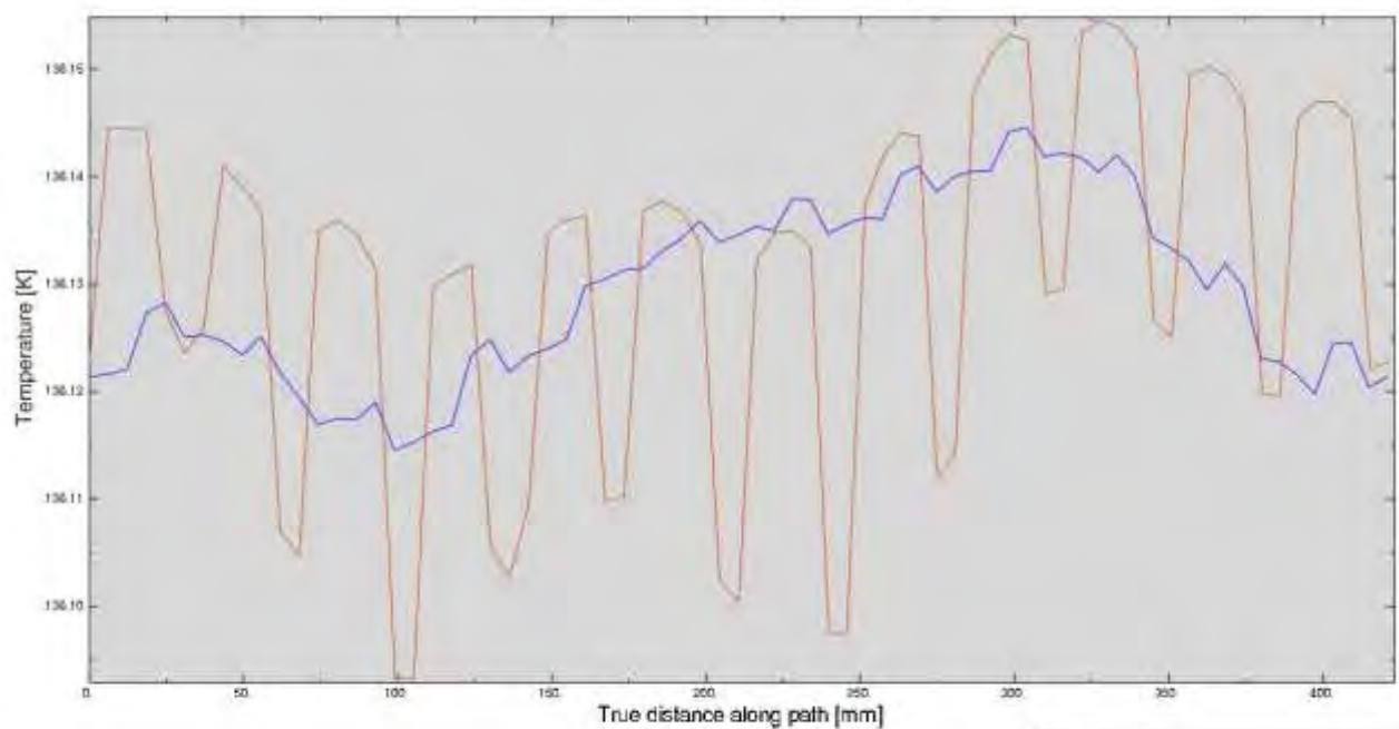
Job 12 CoLA temperature along external edge
