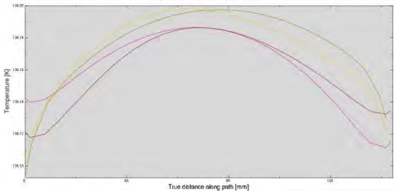
Job 12 CoLA temperature along diameters
