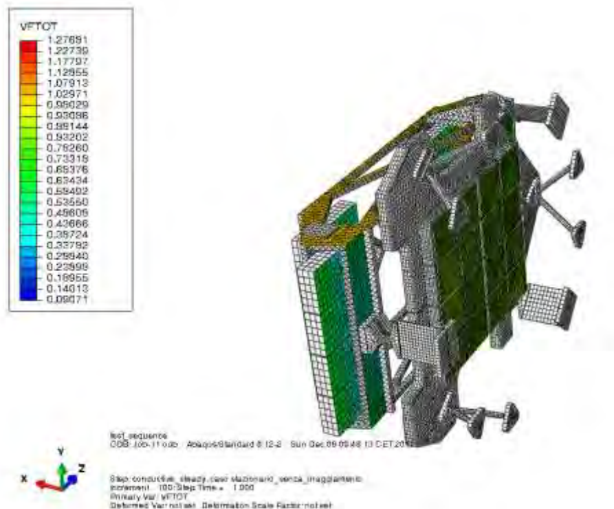
Figure 13-24 Sidecars and Detectors view factor
