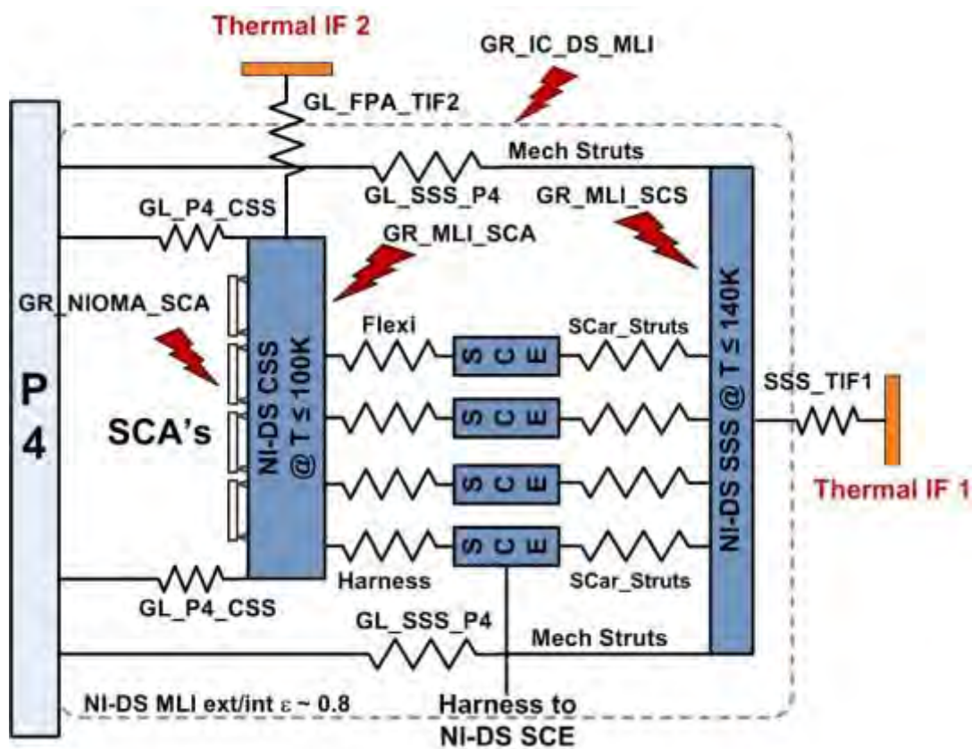
Figure 4-5. NI-DS thermal scheme
