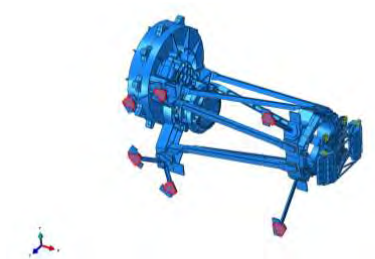
Figure 9-8 Bipods Thermal boundary condition surfaces
