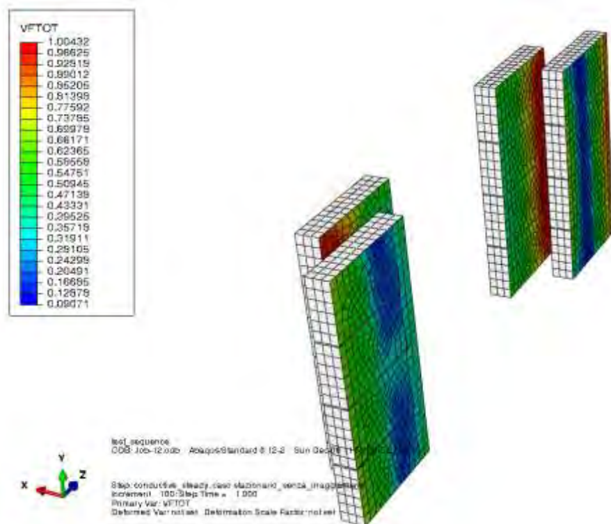
Figure 13-97 Sidcars view factor
