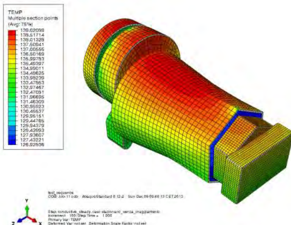
Figure 13-40 Wheels and lenses temperature distribution [K]
