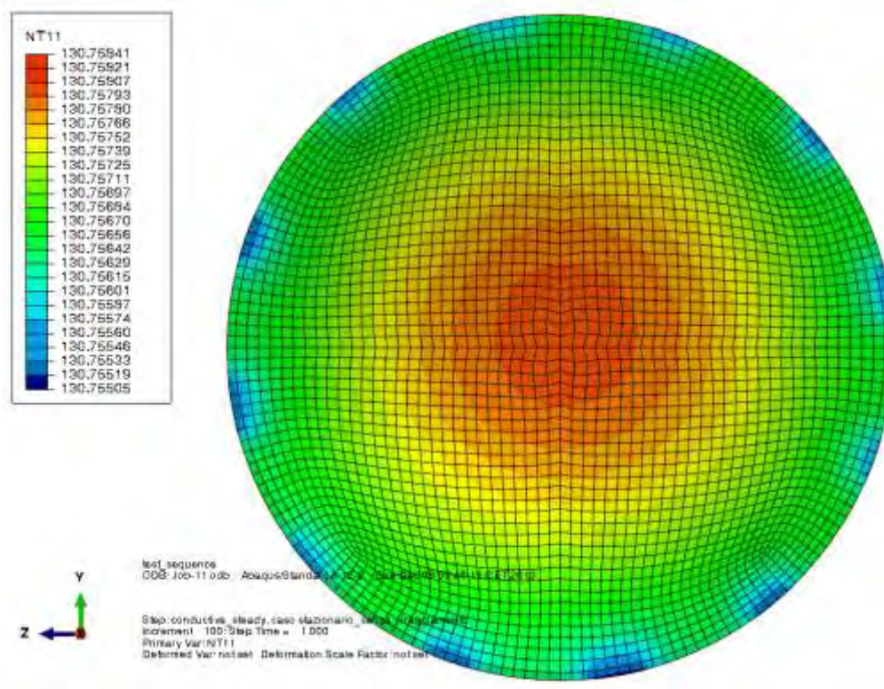
Figure 13-7 CaLA Lens 1 back temperature distribution [K]
