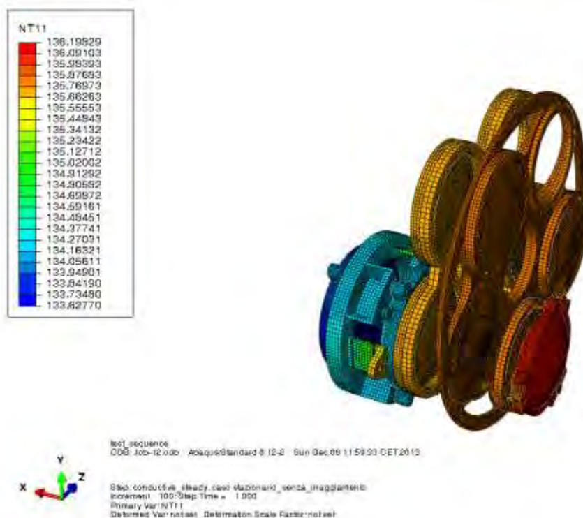
Figure 13-88 NI-OA lenses temperature distribution [K]
