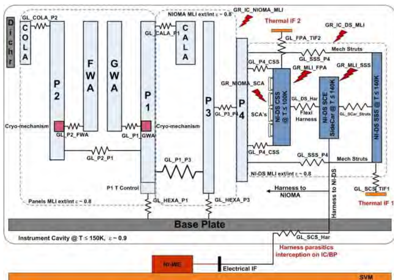
Figure 4-1. NISP thermal concept
